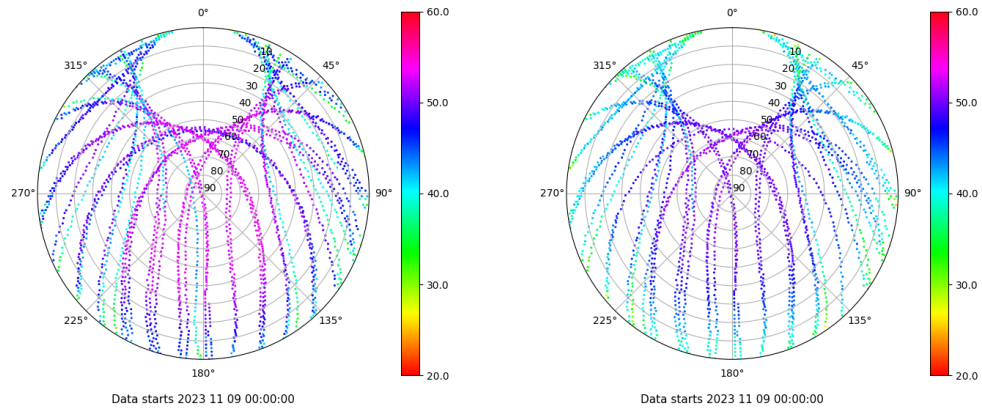
Skyplot for station ALBA. Signal to Noise S1C Data file ALBA00ESP_R_2023313.xtr Skyplot for station ALBA. Signal to Noise S2C Data file ALBA00ESP_R_2023313.xtr
