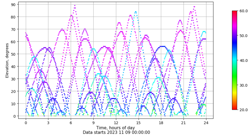
Time-elevation plot for station ALBA. Signal to Noise S1C Data file ALBA00ESP_R_2023313.xtr
