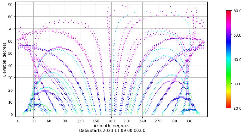
Azimuth-elevation plot for station ALBA. Signal to Noise S1C Data file ALBA00ESP_R_2023313.xtr
