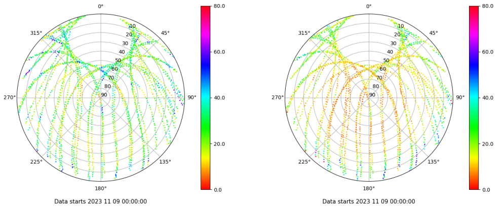
Skyplot for station ALBA. Parameter M1C Data file ALBA00ESP_R_2023313.xtr Skyplot for station ALBA. Parameter M2C Data file ALBA00ESP_R_2023313.xtr
