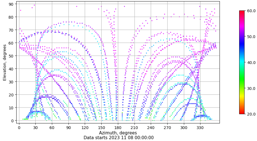
Azimuth-elevation plot for station ALBA. Signal to Noise S1C Data file ALBA00ESP_R_2023312.xtr
