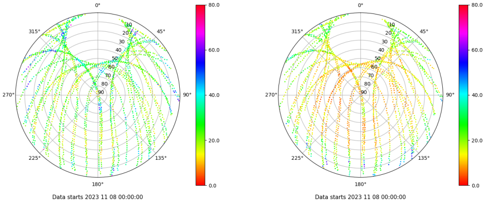
Skyplot for station ALBA. Parameter M1C Data file ALBA00ESP_R_2023312.xtr Skyplot for station ALBA. Parameter M2C Data file ALBA00ESP_R_2023312.xtr
