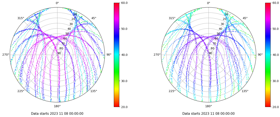
Skyplot for station ALBA. Signal to Noise S1C Data file ALBA00ESP_R_2023312.xtr Skyplot for station ALBA. Signal to Noise S2C Data file ALBA00ESP_R_2023312.xtr
