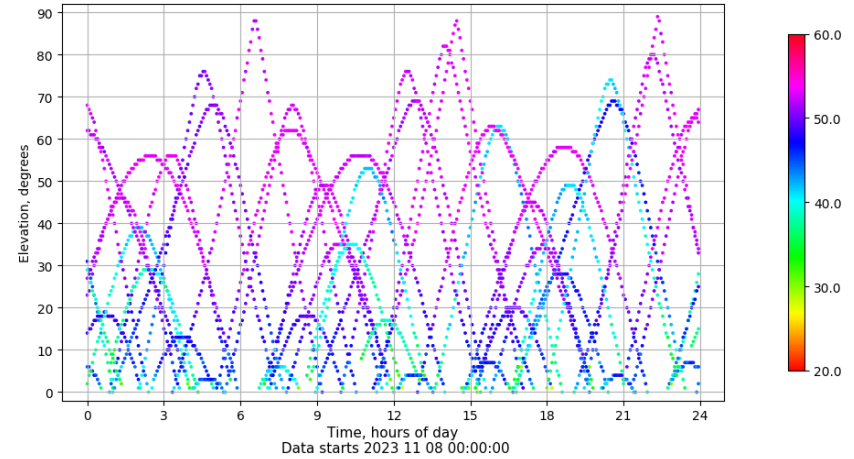
Time-elevation plot for station ALBA. Signal to Noise S1C Data file ALBA00ESP_R_2023312.xtr
