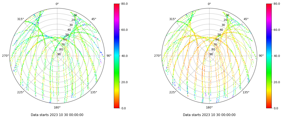
Skyplot for station ALBA. Parameter M1C Data file ALBA00ESP_R_2023303.xtr Skyplot for station ALBA. Parameter M2C Data file ALBA00ESP_R_2023303.xtr
