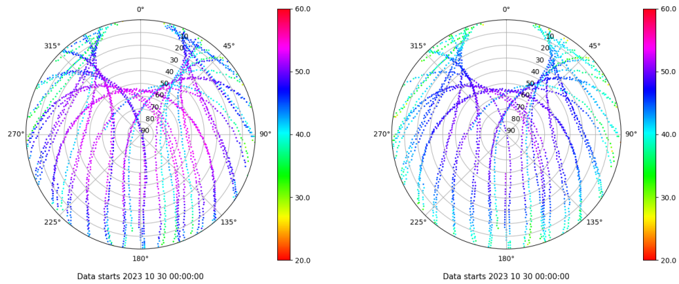
Skyplot for station ALBA. Signal to Noise S1C Data file ALBA00ESP_R_2023303.xtr Skyplot for station ALBA. Signal to Noise S2C Data file ALBA00ESP_R_2023303.xtr
