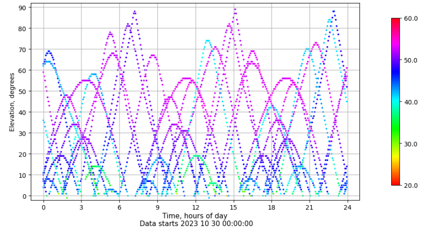
Time-elevation plot for station ALBA. Signal to Noise S1C Data file ALBA00ESP_R_2023303.xtr
