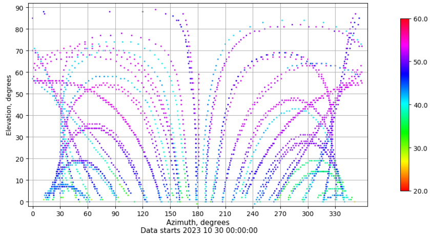
Azimuth-elevation plot for station ALBA. Signal to Noise S1C Data file ALBA00ESP_R_2023303.xtr
