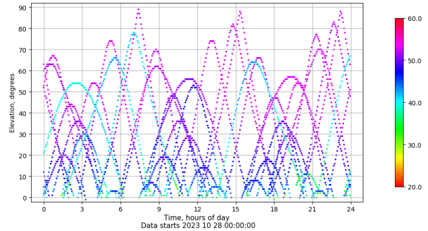
Time-elevation plot for station ALBA. Signal to Noise S1C Data file ALBA00ESP_R_2023301.xtr
