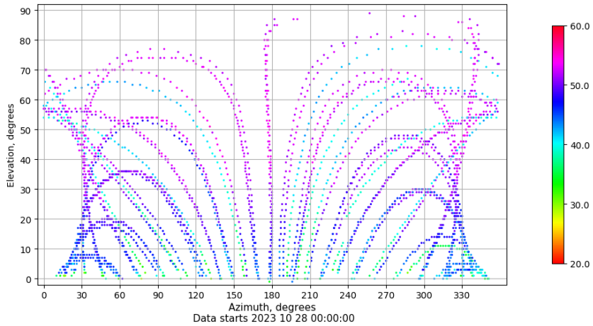
Azimuth-elevation plot for station ALBA. Signal to Noise S1C Data file ALBA00ESP_R_2023301.xtr
