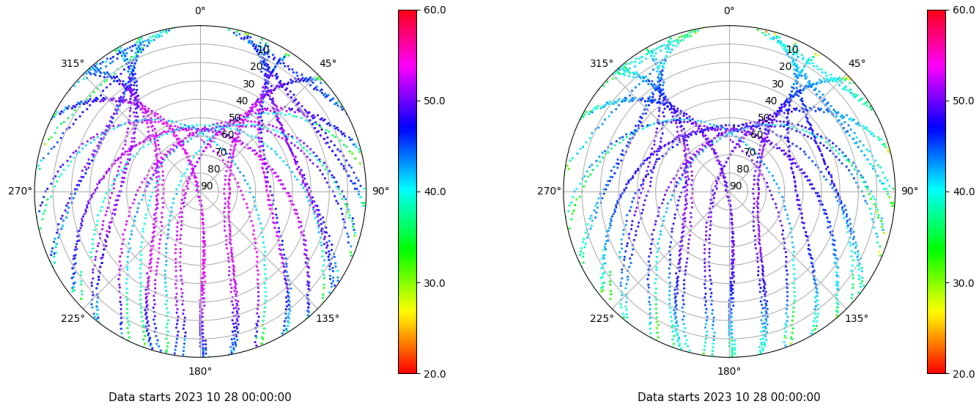
Skyplot for station ALBA. Signal to Noise S1C Data file ALBA00ESP_R_2023301.xtr Skyplot for station ALBA. Signal to Noise S2C Data file ALBA00ESP_R_2023301.xtr
