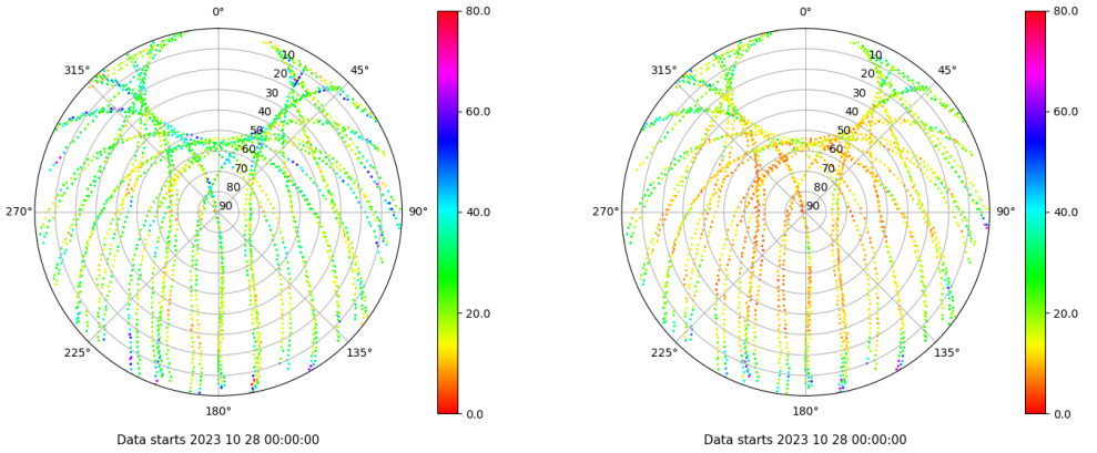
Skyplot for station ALBA. Parameter M1C Data file ALBA00ESP_R_2023301.xtr Skyplot for station ALBA. Parameter M2C Data file ALBA00ESP_R_2023301.xtr
