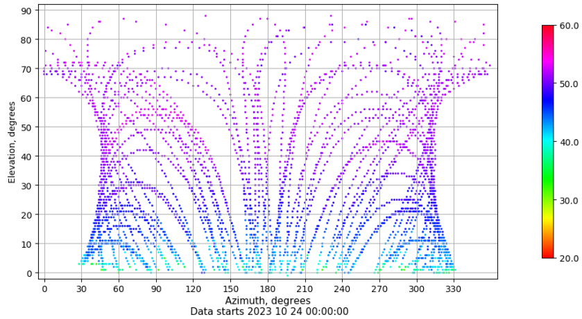
Azimuth-elevation plot for station ALBA. Signal to Noise S1C Data file ALBA00ESP_R_2023297.xtr
