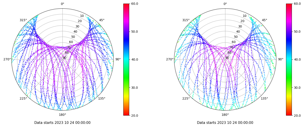
Skyplot for station ALBA. Signal to Noise S1C Data file ALBA00ESP_R_2023297.xtr Skyplot for station ALBA. Signal to Noise S2S Data file ALBA00ESP_R_2023297.xtr
