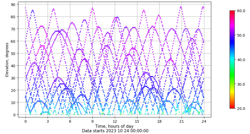
Time-elevation plot for station ALBA. Signal to Noise S1C Data file ALBA00ESP_R_2023297.xtr
