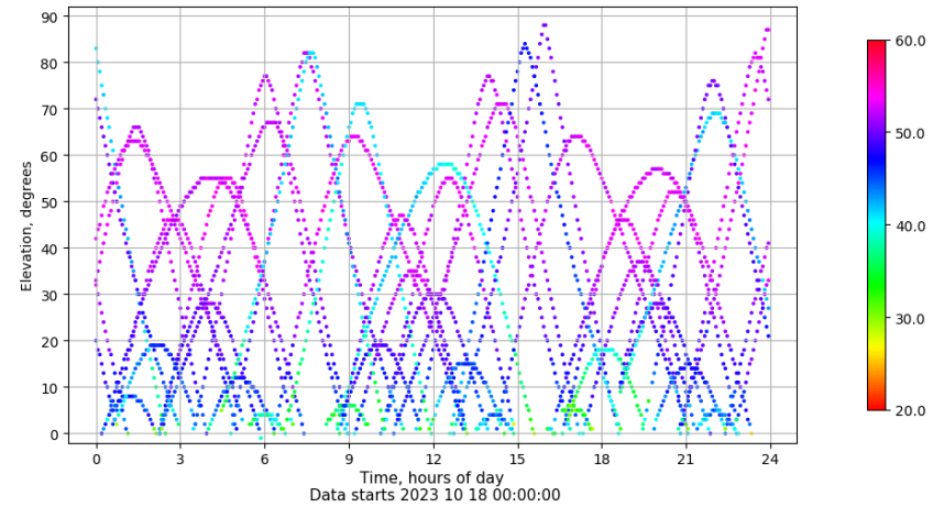
Time-elevation plot for station ALBA. Signal to Noise S1C Data file ALBA00ESP_R_2023291.xtr
