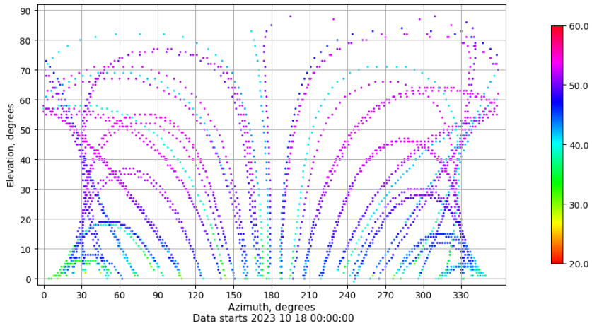
Azimuth-elevation plot for station ALBA. Signal to Noise S1C Data file ALBA00ESP_R_2023291.xtr
