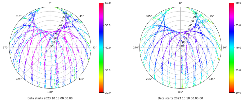
Skyplot for station ALBA. Signal to Noise S1C Data file ALBA00ESP_R_2023291.xtr Skyplot for station ALBA. Signal to Noise S2C Data file ALBA00ESP_R_2023291.xtr
