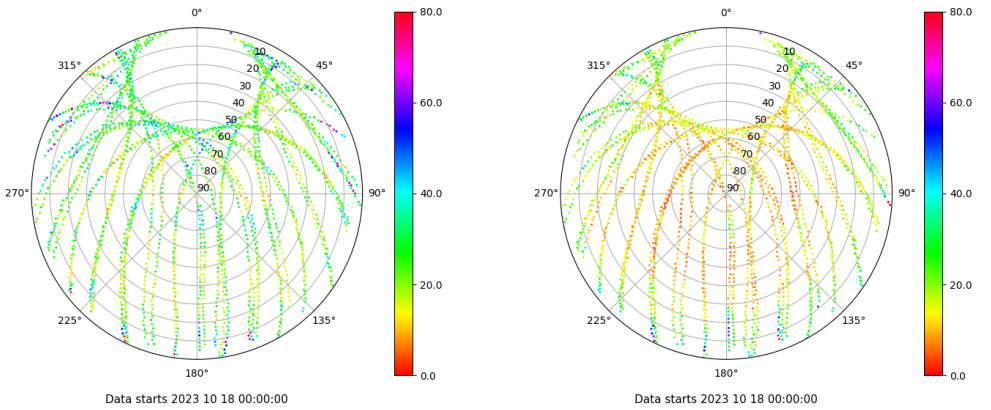
Skyplot for station ALBA. Parameter M1C Data file ALBA00ESP_R_2023291.xtr Skyplot for station ALBA. Parameter M2C Data file ALBA00ESP_R_2023291.xtr
