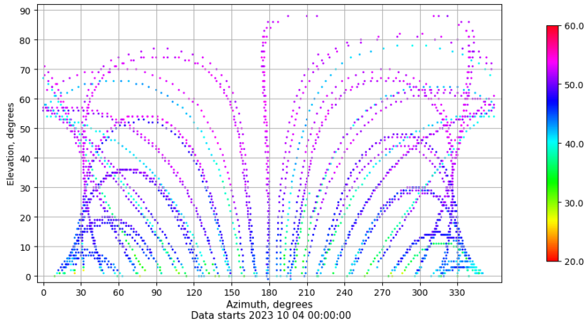
Azimuth-elevation plot for station ALBA. Signal to Noise S1C Data file ALBA00ESP_R_2023277.xtr
