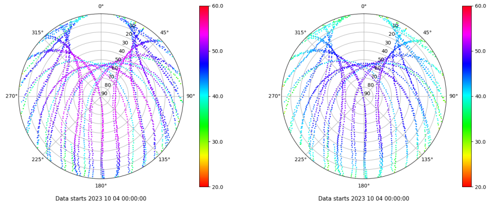
Skyplot for station ALBA. Signal to Noise S1C Data file ALBA00ESP_R_2023277.xtr Skyplot for station ALBA. Signal to Noise S2C Data file ALBA00ESP_R_2023277.xtr
