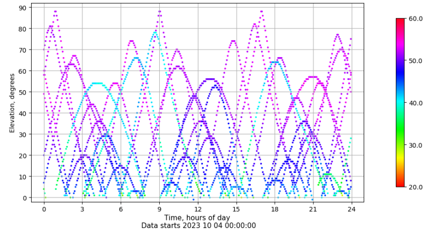
Time-elevation plot for station ALBA. Signal to Noise S1C Data file ALBA00ESP_R_2023277.xtr
