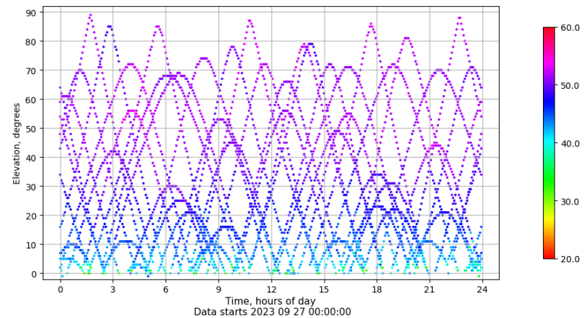
Time-elevation plot for station ALBA. Signal to Noise S1C Data file ALBA00ESP_R_2023270.xtr
