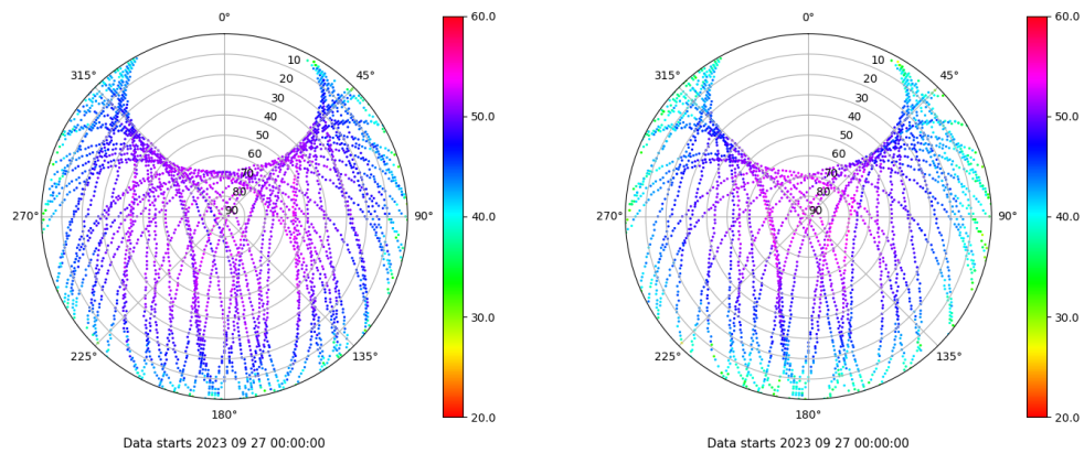
Skyplot for station ALBA. Signal to Noise S1C Data file ALBA00ESP_R_2023270.xtr Skyplot for station ALBA. Signal to Noise S2S Data file ALBA00ESP_R_2023270.xtr
