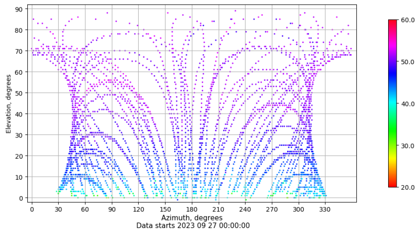
Azimuth-elevation plot for station ALBA. Signal to Noise S1C Data file ALBA00ESP_R_2023270.xtr
