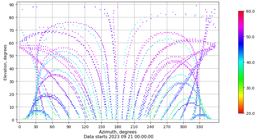
Azimuth-elevation plot for station ALBA. Signal to Noise S1C Data file ALBA00ESP_R_2023264.xtr
