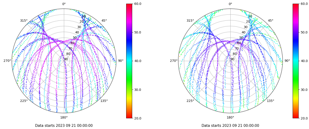
Skyplot for station ALBA. Signal to Noise S1C Data file ALBA00ESP_R_2023264.xtr Skyplot for station ALBA. Signal to Noise S2C Data file ALBA00ESP_R_2023264.xtr
