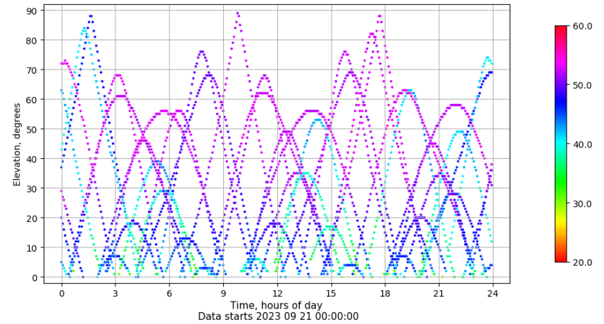
Time-elevation plot for station ALBA. Signal to Noise S1C Data file ALBA00ESP_R_2023264.xtr
