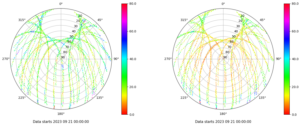
Skyplot for station ALBA. Parameter M1C Data file ALBA00ESP_R_2023264.xtr Skyplot for station ALBA. Parameter M2C Data file ALBA00ESP_R_2023264.xtr
