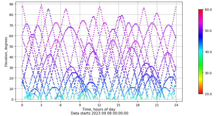
Time-elevation plot for station ALBA. Signal to Noise S1C Data file ALBA00ESP_R_2023251.xtr
