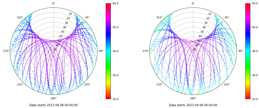
Skyplot for station ALBA. Signal to Noise S1C Data file ALBA00ESP_R_2023251.xtr Skyplot for station ALBA. Signal to Noise S2S Data file ALBA00ESP_R_2023251.xtr
