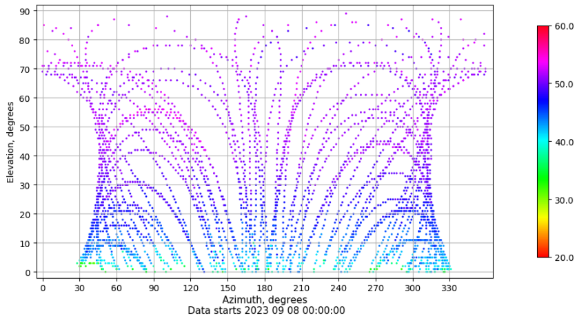
Azimuth-elevation plot for station ALBA. Signal to Noise S1C Data file ALBA00ESP_R_2023251.xtr
