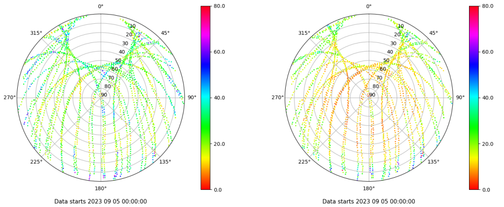
Skyplot for station ALBA. Parameter M1C Data file ALBA00ESP_R_2023248.xtr Skyplot for station ALBA. Parameter M2C Data file ALBA00ESP_R_2023248.xtr
