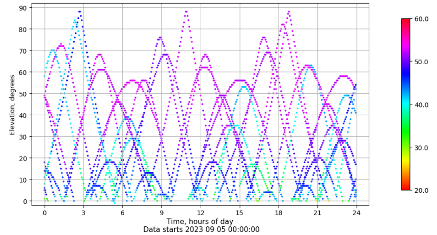
Time-elevation plot for station ALBA. Signal to Noise S1C Data file ALBA00ESP_R_2023248.xtr
