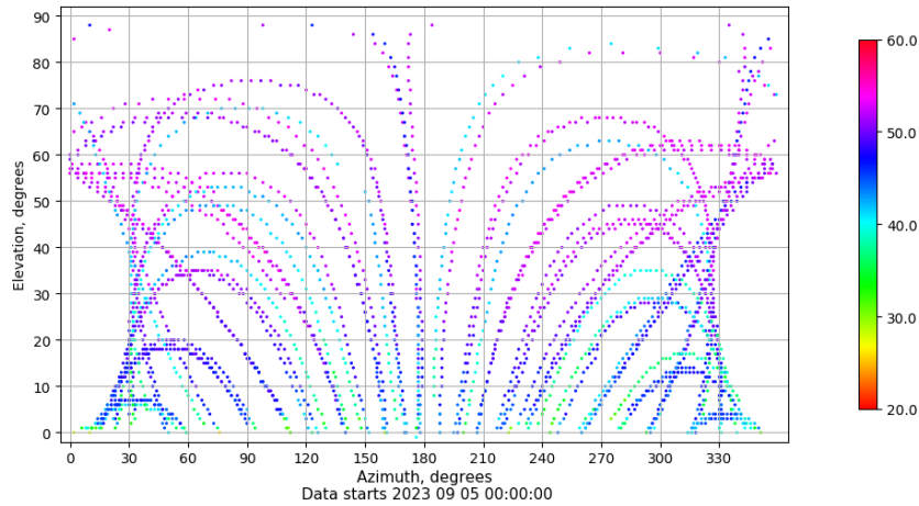
Azimuth-elevation plot for station ALBA. Signal to Noise S1C Data file ALBA00ESP_R_2023248.xtr
