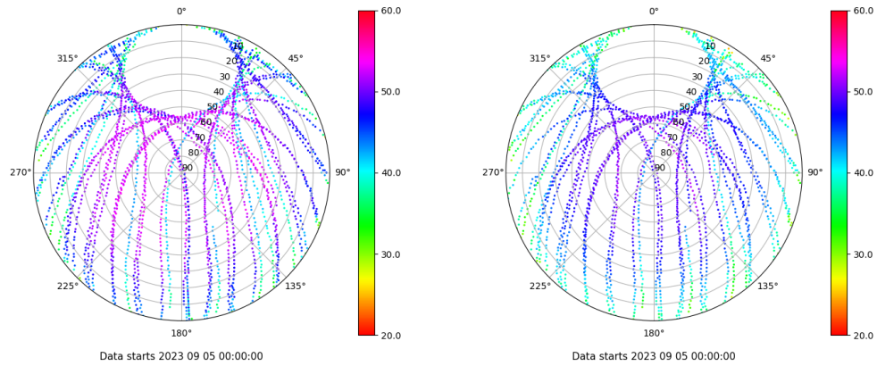
Skyplot for station ALBA. Signal to Noise S1C Data file ALBA00ESP_R_2023248.xtr Skyplot for station ALBA. Signal to Noise S2C Data file ALBA00ESP_R_2023248.xtr
