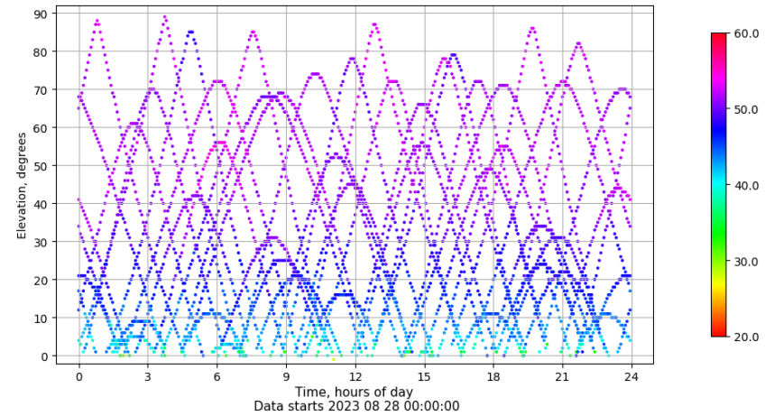
Time-elevation plot for station ALBA. Signal to Noise S1C Data file ALBA00ESP_R_2023240.xtr
