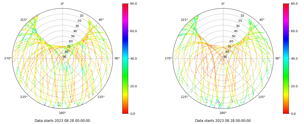
Skyplot for station ALBA. Parameter M1C Data file ALBA00ESP_R_2023240.xtr Skyplot for station ALBA. Parameter M2S Data file ALBA00ESP_R_2023240.xtr
