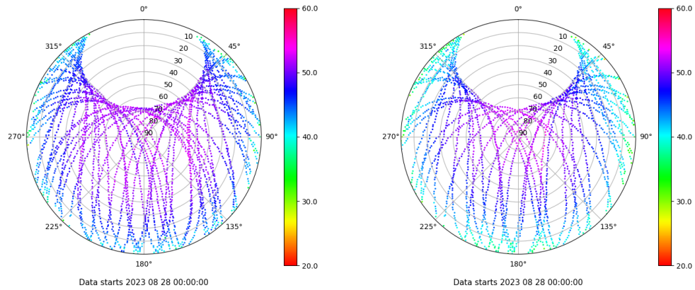
Skyplot for station ALBA. Signal to Noise S1C Data file ALBA00ESP_R_2023240.xtr Skyplot for station ALBA. Signal to Noise S2S Data file ALBA00ESP_R_2023240.xtr
