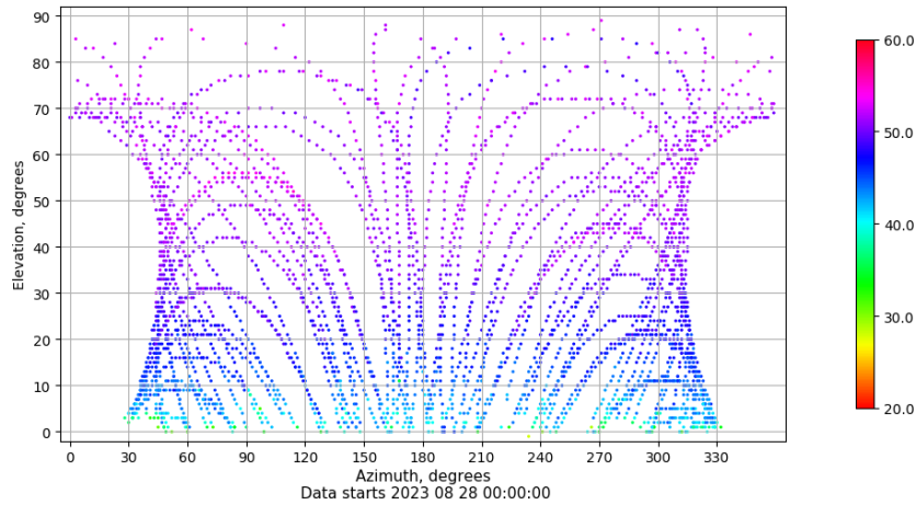
Azimuth-elevation plot for station ALBA. Signal to Noise S1C Data file ALBA00ESP_R_2023240.xtr
