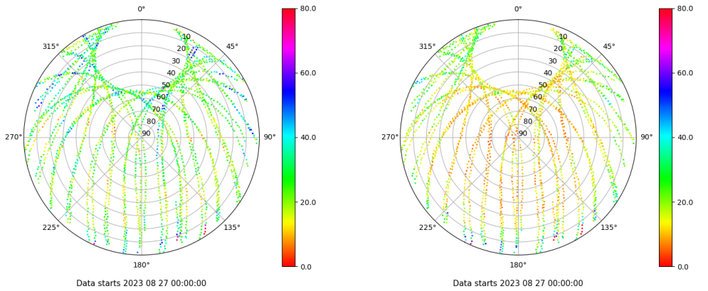
Skyplot for station ALBA. Parameter M1C Data file ALBA00ESP_R_2023239.xtr Skyplot for station ALBA. Parameter M2C Data file ALBA00ESP_R_2023239.xtr
