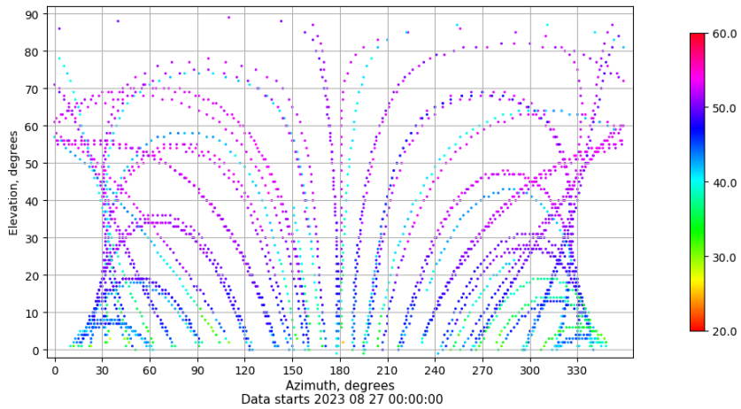
Azimuth-elevation plot for station ALBA. Signal to Noise S1C Data file ALBA00ESP_R_2023239.xtr
