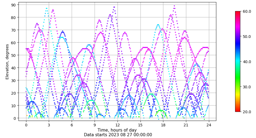
Time-elevation plot for station ALBA. Signal to Noise S1C Data file ALBA00ESP_R_2023239.xtr
