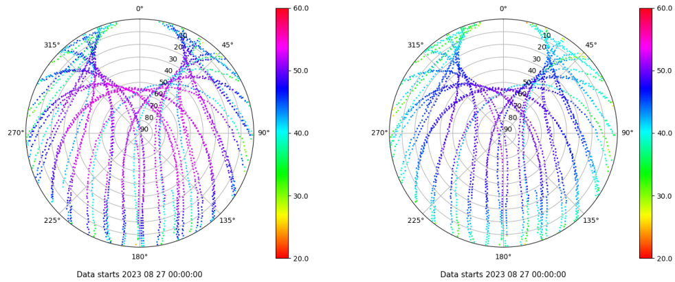
Skyplot for station ALBA. Signal to Noise S1C Data file ALBA00ESP_R_2023239.xtr Skyplot for station ALBA. Signal to Noise S2C Data file ALBA00ESP_R_2023239.xtr
