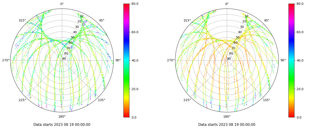
Skyplot for station ALBA. Parameter M1C Data file ALBA00ESP_R_2023231.xtr Skyplot for station ALBA. Parameter M2C Data file ALBA00ESP_R_2023231.xtr
