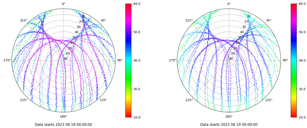
Skyplot for station ALBA. Signal to Noise S1C Data file ALBA00ESP_R_2023231.xtr Skyplot for station ALBA. Signal to Noise S2C Data file ALBA00ESP_R_2023231.xtr
