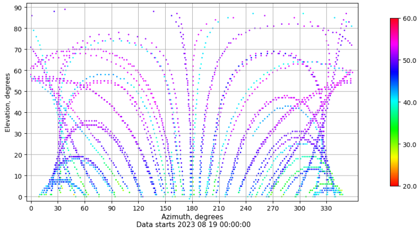
Azimuth-elevation plot for station ALBA. Signal to Noise S1C Data file ALBA00ESP_R_2023231.xtr
