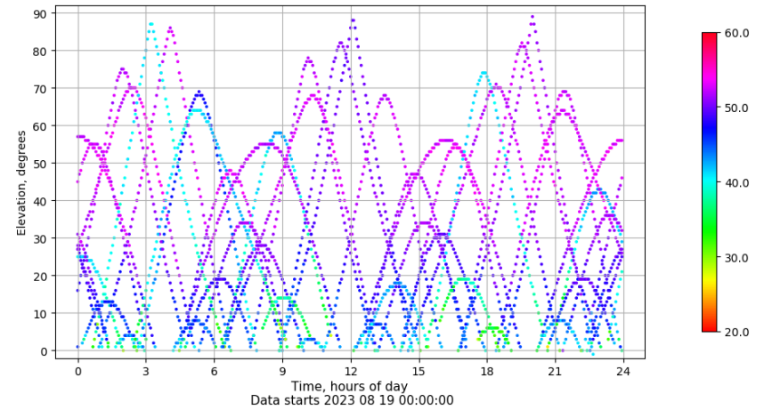
Time-elevation plot for station ALBA. Signal to Noise S1C Data file ALBA00ESP_R_2023231.xtr
