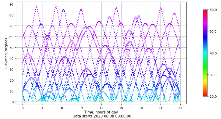
Time-elevation plot for station ALBA. Signal to Noise S1C Data file ALBA00ESP_R_2023220.xtr
