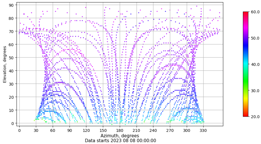
Azimuth-elevation plot for station ALBA. Signal to Noise S1C Data file ALBA00ESP_R_2023220.xtr
