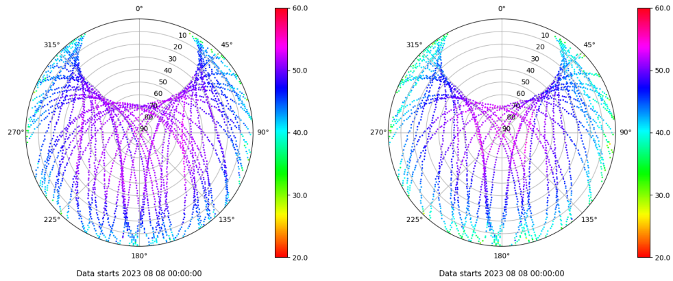
Skyplot for station ALBA. Signal to Noise S1C Data file ALBA00ESP_R_2023220.xtr Skyplot for station ALBA. Signal to Noise S2S Data file ALBA00ESP_R_2023220.xtr
