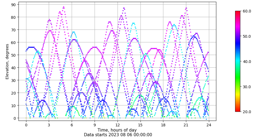
Time-elevation plot for station ALBA. Signal to Noise S1C Data file ALBA00ESP_R_2023218.xtr
