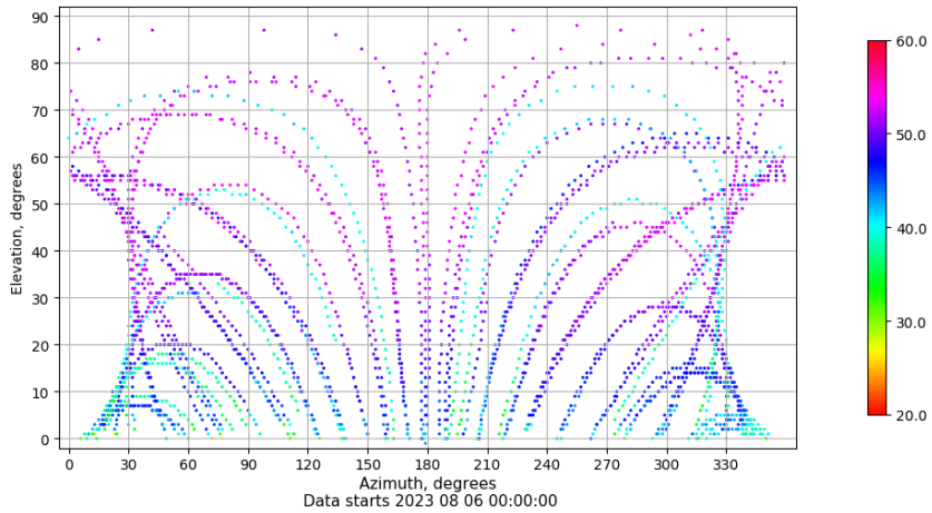
Azimuth-elevation plot for station ALBA. Signal to Noise S1C Data file ALBA00ESP_R_2023218.xtr
