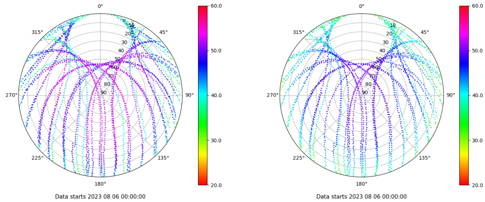
Skyplot for station ALBA. Signal to Noise S1C Data file ALBA00ESP_R_2023218.xtr Skyplot for station ALBA. Signal to Noise S2C Data file ALBA00ESP_R_2023218.xtr
