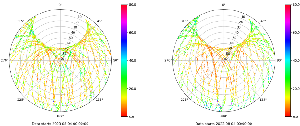
Skyplot for station ALBA. Parameter M1C Data file ALBA00ESP_R_2023216.xtr Skyplot for station ALBA. Parameter M2S Data file ALBA00ESP_R_2023216.xtr
