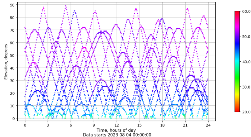
Time-elevation plot for station ALBA. Signal to Noise S1C Data file ALBA00ESP_R_2023216.xtr
