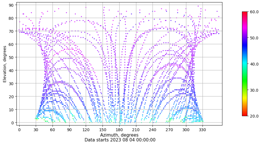
Azimuth-elevation plot for station ALBA. Signal to Noise S1C Data file ALBA00ESP_R_2023216.xtr
