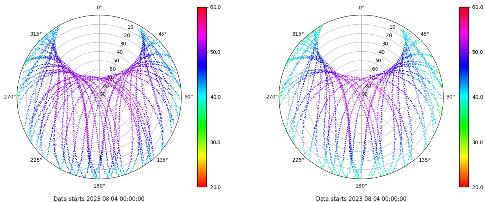
Skyplot for station ALBA. Signal to Noise S1C Data file ALBA00ESP_R_2023216.xtr Skyplot for station ALBA. Signal to Noise S2S Data file ALBA00ESP_R_2023216.xtr
