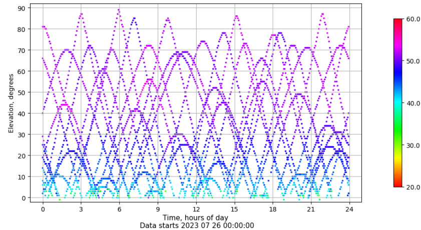
Time-elevation plot for station ALBA. Signal to Noise S1C Data file ALBA00ESP_R_2023207.xtr
