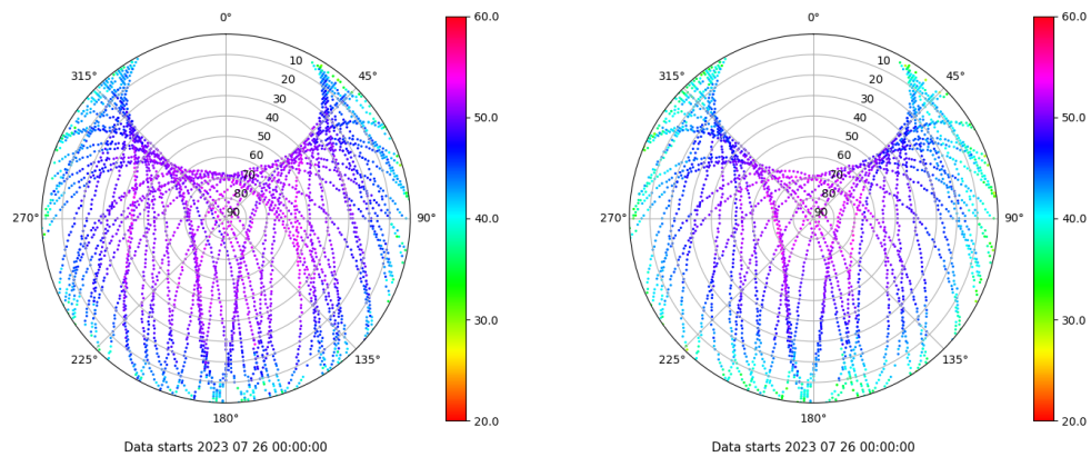
Skyplot for station ALBA. Signal to Noise S1C Data file ALBA00ESP_R_2023207.xtr Skyplot for station ALBA. Signal to Noise S2S Data file ALBA00ESP_R_2023207.xtr
