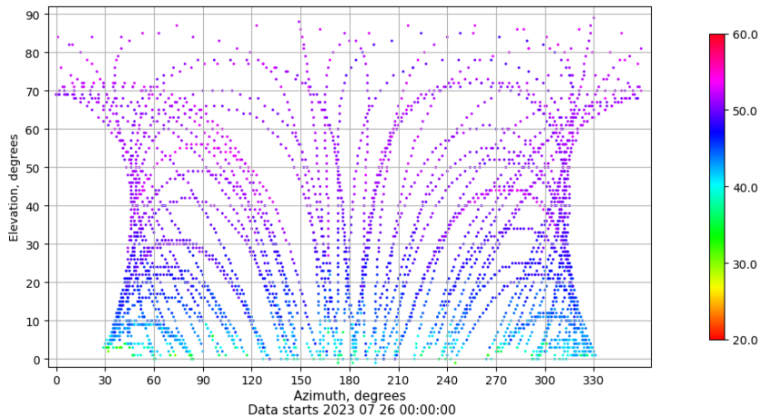
Azimuth-elevation plot for station ALBA. Signal to Noise S1C Data file ALBA00ESP_R_2023207.xtr
