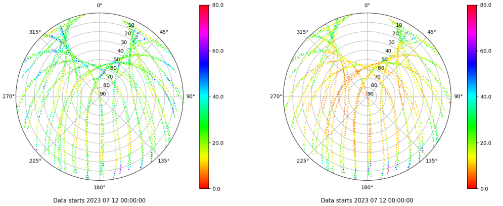
Skyplot for station ALBA. Parameter M1C Data file ALBA00ESP_R_2023193.xtr Skyplot for station ALBA. Parameter M2C Data file ALBA00ESP_R_2023193.xtr
