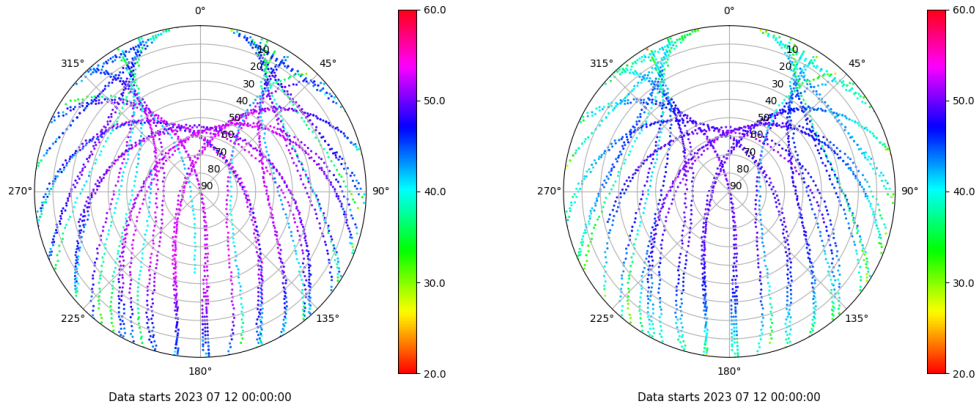
Skyplot for station ALBA. Signal to Noise S1C Data file ALBA00ESP_R_2023193.xtr Skyplot for station ALBA. Signal to Noise S2C Data file ALBA00ESP_R_2023193.xtr
