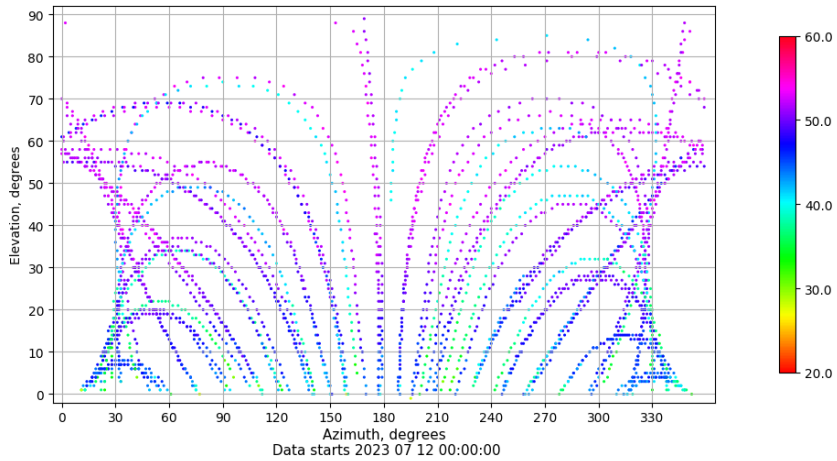
Azimuth-elevation plot for station ALBA. Signal to Noise S1C Data file ALBA00ESP_R_2023193.xtr
