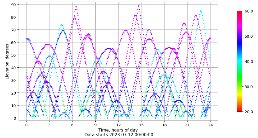
Time-elevation plot for station ALBA. Signal to Noise S1C Data file ALBA00ESP_R_2023193.xtr
