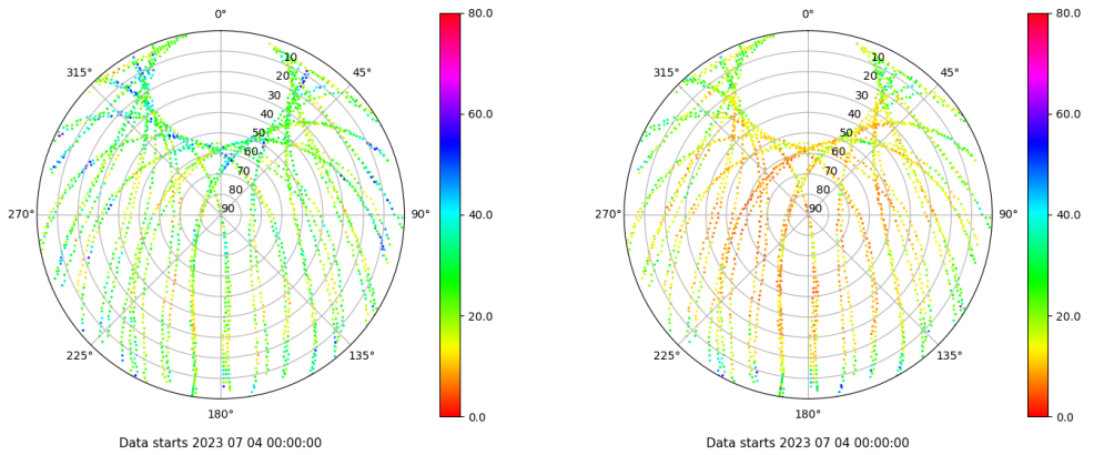
Skyplot for station ALBA. Parameter M1C Data file ALBA00ESP_R_2023185.xtr Skyplot for station ALBA. Parameter M2C Data file ALBA00ESP_R_2023185.xtr
