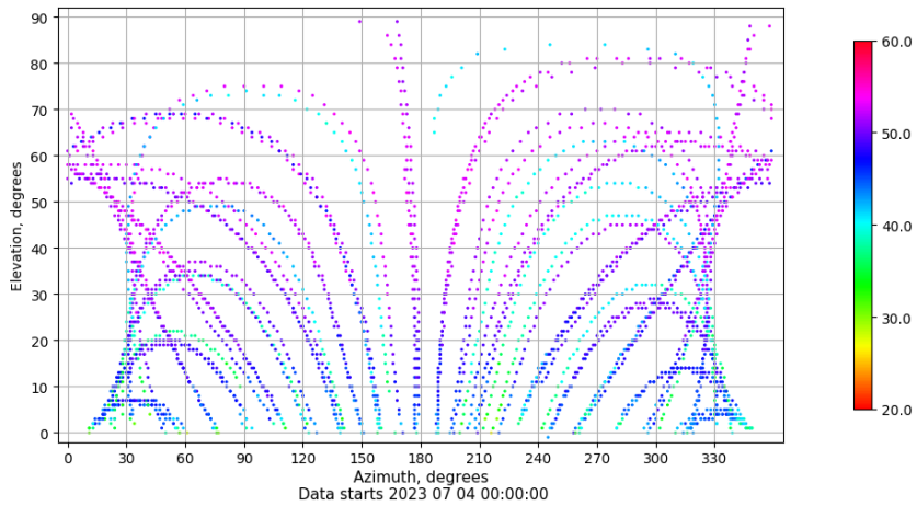
Azimuth-elevation plot for station ALBA. Signal to Noise S1C Data file ALBA00ESP_R_2023185.xtr
