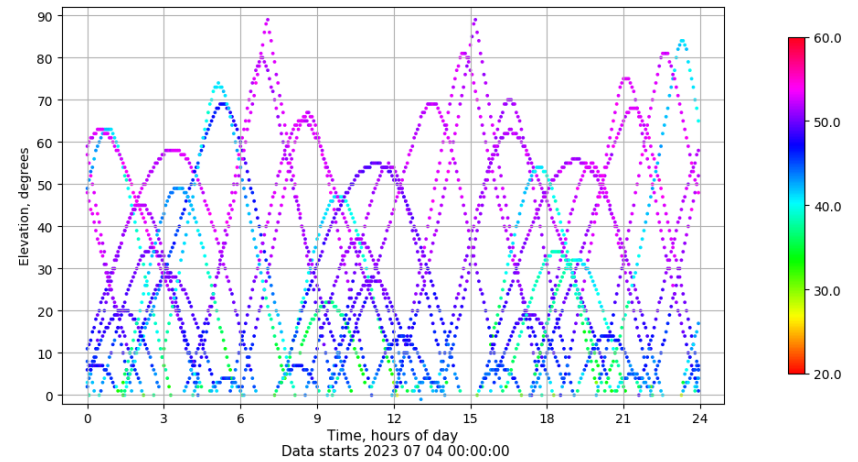
Time-elevation plot for station ALBA. Signal to Noise S1C Data file ALBA00ESP_R_2023185.xtr
