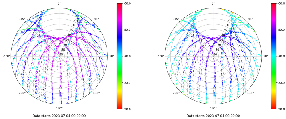
Skyplot for station ALBA. Signal to Noise S1C Data file ALBA00ESP_R_2023185.xtr Skyplot for station ALBA. Signal to Noise S2C Data file ALBA00ESP_R_2023185.xtr
