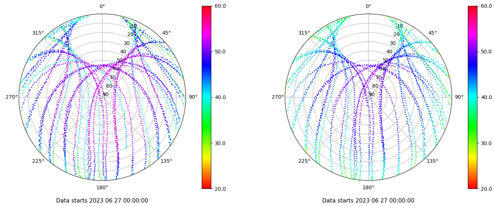
Skyplot for station ALBA. Signal to Noise S1C Data file ALBA00ESP_R_2023178.xtr Skyplot for station ALBA. Signal to Noise S2C Data file ALBA00ESP_R_2023178.xtr
