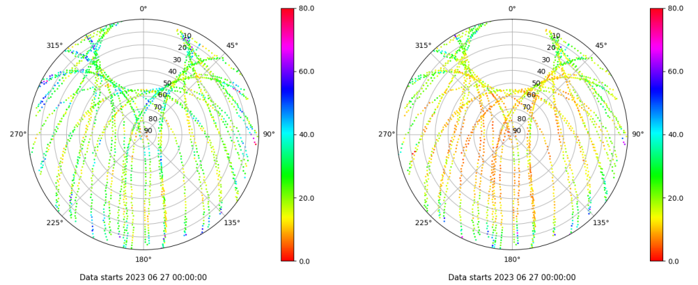
Skyplot for station ALBA. Parameter M1C Data file ALBA00ESP_R_2023178.xtr Skyplot for station ALBA. Parameter M2C Data file ALBA00ESP_R_2023178.xtr
