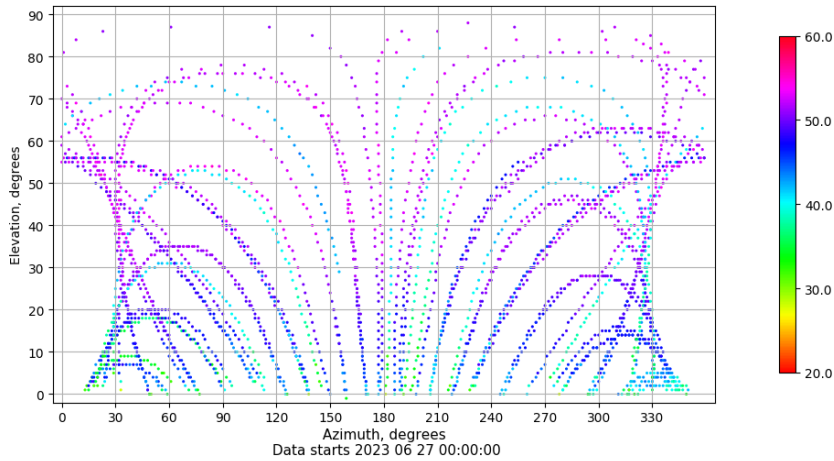
Azimuth-elevation plot for station ALBA. Signal to Noise S1C Data file ALBA00ESP_R_2023178.xtr
