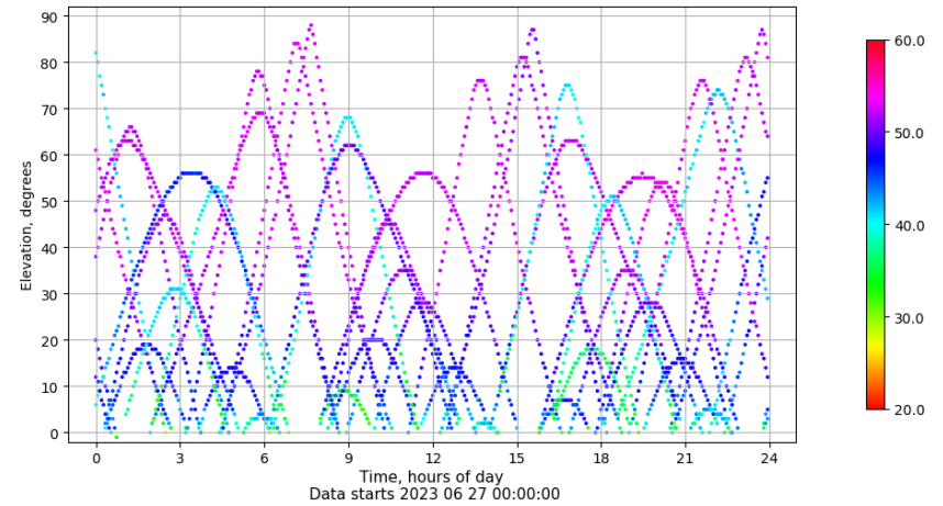
Time-elevation plot for station ALBA. Signal to Noise S1C Data file ALBA00ESP_R_2023178.xtr
