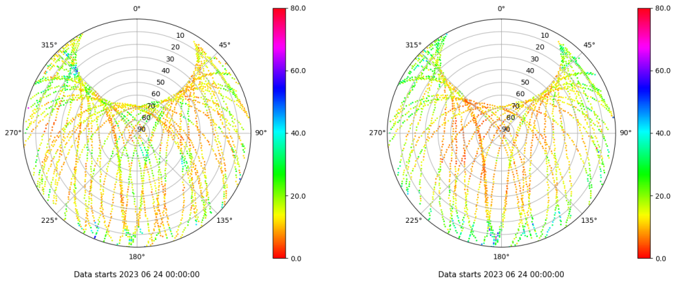
Skyplot for station ALBA. Parameter M1C Data file ALBA00ESP_R_2023175.xtr Skyplot for station ALBA. Parameter M2S Data file ALBA00ESP_R_2023175.xtr
