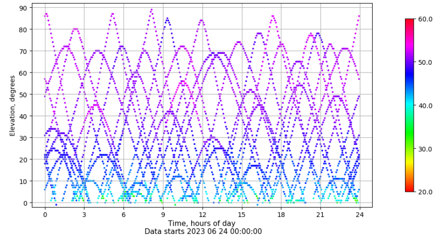
Time-elevation plot for station ALBA. Signal to Noise S1C Data file ALBA00ESP_R_2023175.xtr
