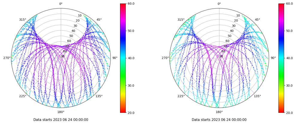
Skyplot for station ALBA. Signal to Noise S1C Data file ALBA00ESP_R_2023175.xtr Skyplot for station ALBA. Signal to Noise S2S Data file ALBA00ESP_R_2023175.xtr
