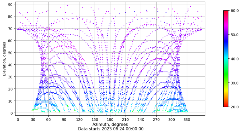
Azimuth-elevation plot for station ALBA. Signal to Noise S1C Data file ALBA00ESP_R_2023175.xtr
