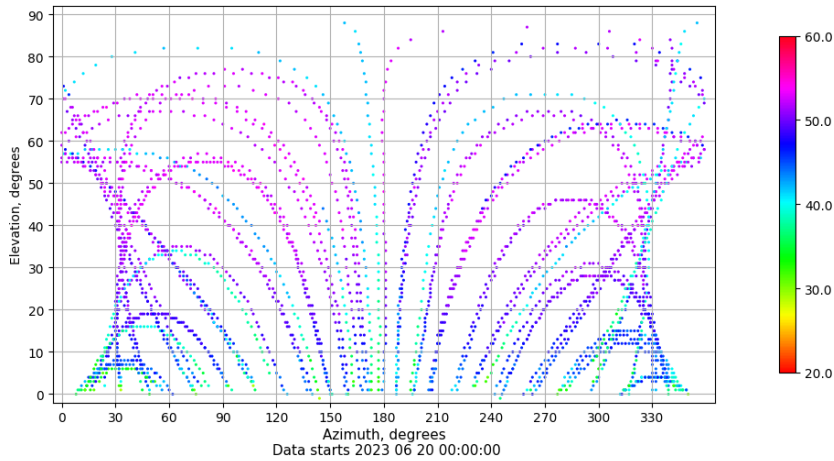
Azimuth-elevation plot for station ALBA. Signal to Noise S1C Data file ALBA00ESP_R_2023171.xtr
