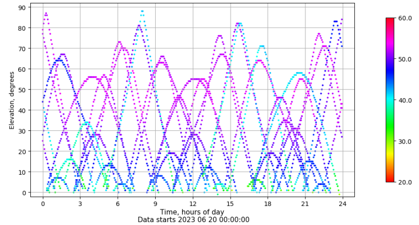
Time-elevation plot for station ALBA. Signal to Noise S1C Data file ALBA00ESP_R_2023171.xtr
