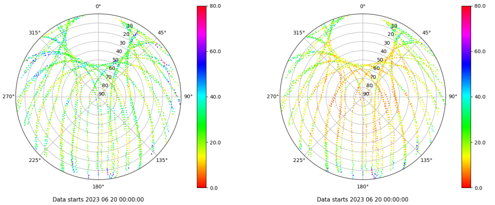
Skyplot for station ALBA. Parameter M1C Data file ALBA00ESP_R_2023171.xtr Skyplot for station ALBA. Parameter M2C Data file ALBA00ESP_R_2023171.xtr
