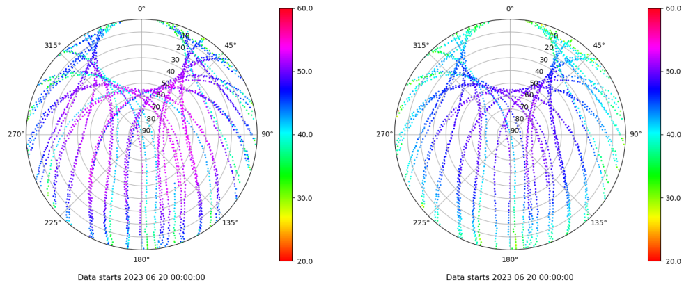
Skyplot for station ALBA. Signal to Noise S1C Data file ALBA00ESP_R_2023171.xtr Skyplot for station ALBA. Signal to Noise S2C Data file ALBA00ESP_R_2023171.xtr
