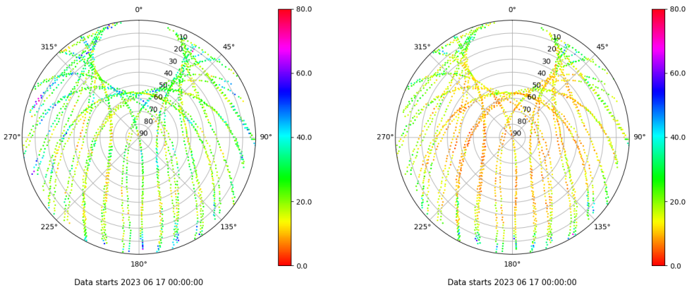
Skyplot for station ALBA. Parameter M1C Data file ALBA00ESP_R_2023168.xtr Skyplot for station ALBA. Parameter M2C Data file ALBA00ESP_R_2023168.xtr
