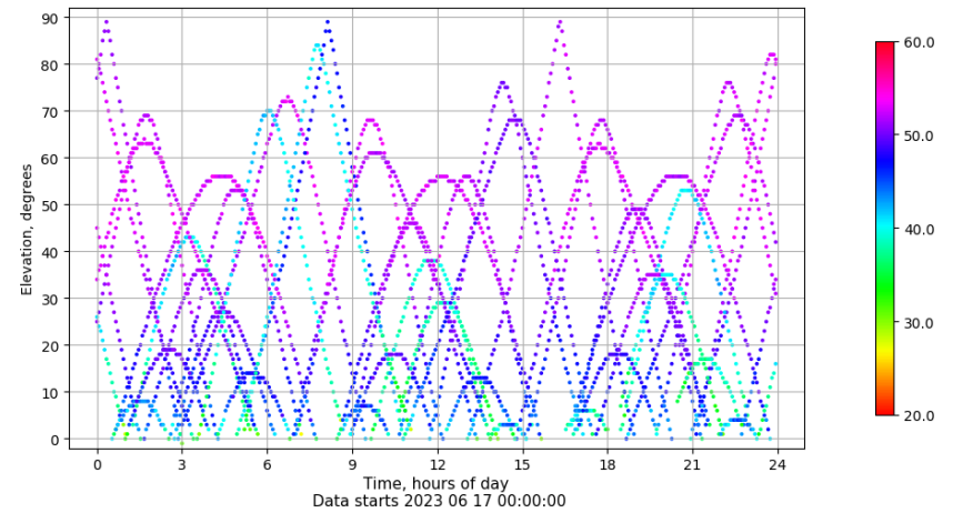
Time-elevation plot for station ALBA. Signal to Noise S1C Data file ALBA00ESP_R_2023168.xtr
