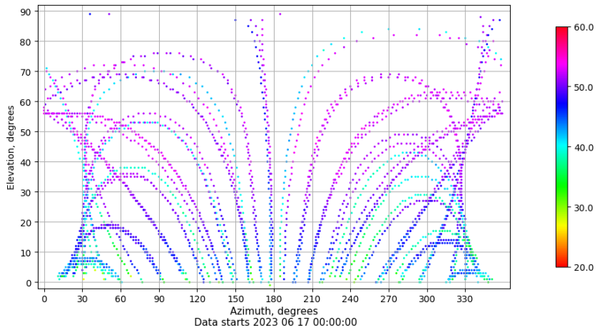
Azimuth-elevation plot for station ALBA. Signal to Noise S1C Data file ALBA00ESP_R_2023168.xtr
