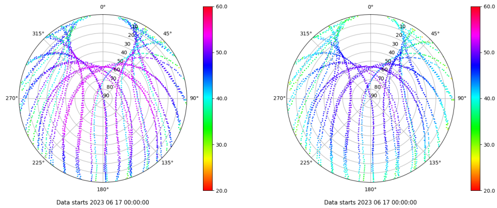
Skyplot for station ALBA. Signal to Noise S1C Data file ALBA00ESP_R_2023168.xtr Skyplot for station ALBA. Signal to Noise S2C Data file ALBA00ESP_R_2023168.xtr
