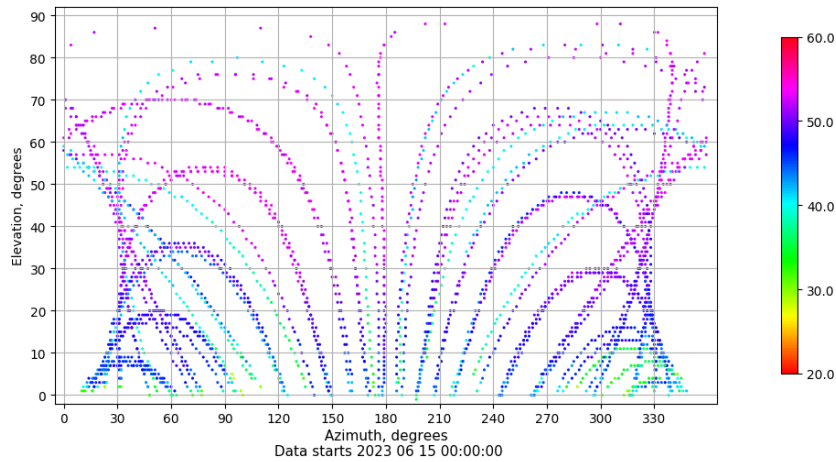
Azimuth-elevation plot for station ALBA. Signal to Noise S1C Data file ALBA00ESP_R_2023166.xtr
