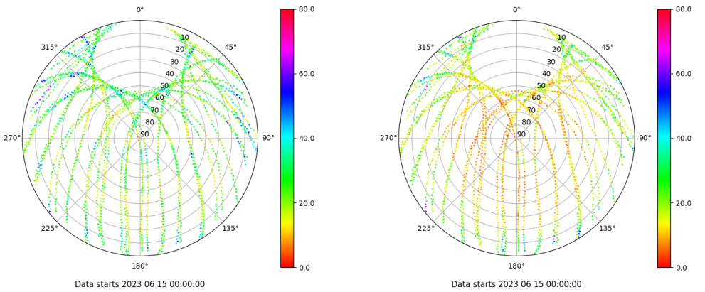
Skyplot for station ALBA. Parameter M1C Data file ALBA00ESP_R_2023166.xtr Skyplot for station ALBA. Parameter M2C Data file ALBA00ESP_R_2023166.xtr
