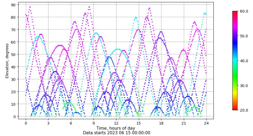
Time-elevation plot for station ALBA. Signal to Noise S1C Data file ALBA00ESP_R_2023166.xtr
