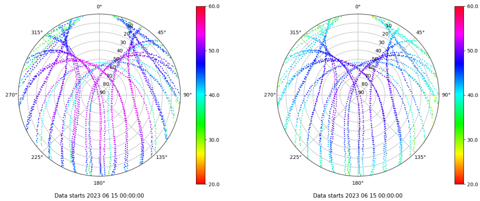
Skyplot for station ALBA. Signal to Noise S1C Data file ALBA00ESP_R_2023166.xtr Skyplot for station ALBA. Signal to Noise S2C Data file ALBA00ESP_R_2023166.xtr
