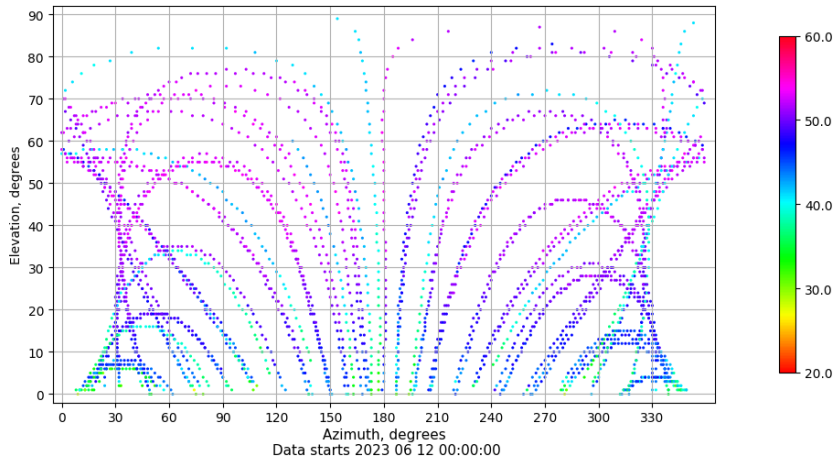
Azimuth-elevation plot for station ALBA. Signal to Noise S1C Data file ALBA00ESP_R_2023163.xtr
