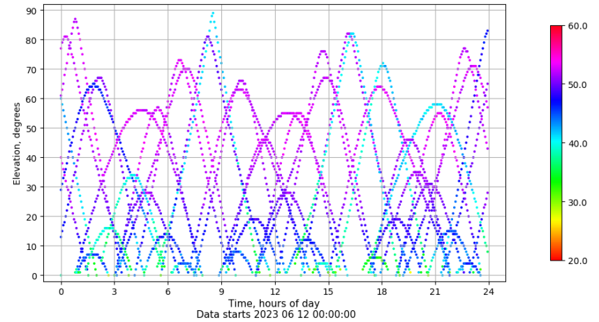
Time-elevation plot for station ALBA. Signal to Noise S1C Data file ALBA00ESP_R_2023163.xtr
