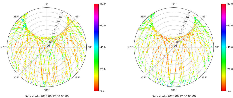
Skyplot for station ALBA. Parameter M1C Data file ALBA00ESP_R_2023163.xtr Skyplot for station ALBA. Parameter M2S Data file ALBA00ESP_R_2023163.xtr
