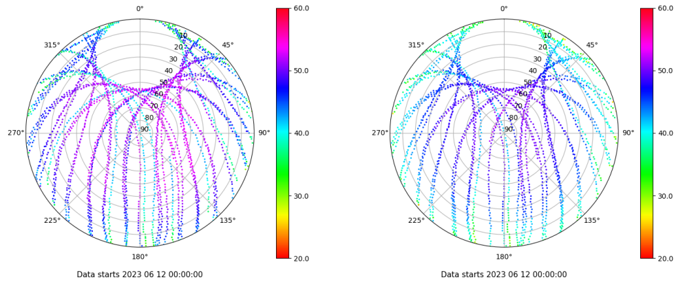
Skyplot for station ALBA. Signal to Noise S1C Data file ALBA00ESP_R_2023163.xtr Skyplot for station ALBA. Signal to Noise S2C Data file ALBA00ESP_R_2023163.xtr
