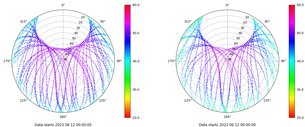
Skyplot for station ALBA. Signal to Noise S1C Data file ALBA00ESP_R_2023163.xtr Skyplot for station ALBA. Signal to Noise S2S Data file ALBA00ESP_R_2023163.xtr
