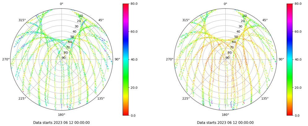
Skyplot for station ALBA. Parameter M1C Data file ALBA00ESP_R_2023163.xtr Skyplot for station ALBA. Parameter M2C Data file ALBA00ESP_R_2023163.xtr
