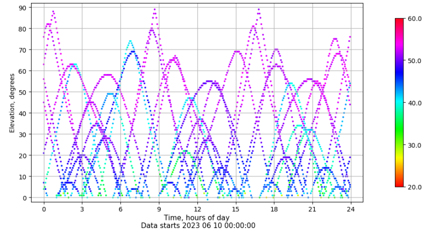
Time-elevation plot for station ALBA. Signal to Noise S1C Data file ALBA00ESP_R_2023161.xtr
