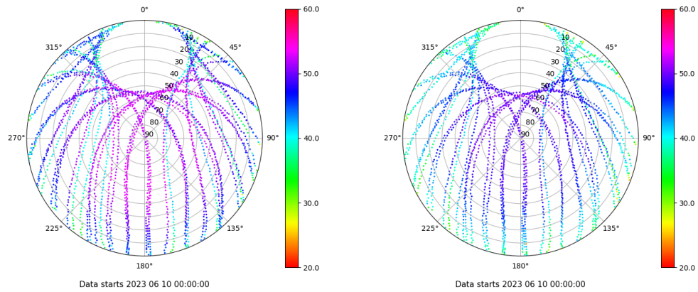
Skyplot for station ALBA. Signal to Noise S1C Data file ALBA00ESP_R_2023161.xtr Skyplot for station ALBA. Signal to Noise S2C Data file ALBA00ESP_R_2023161.xtr
