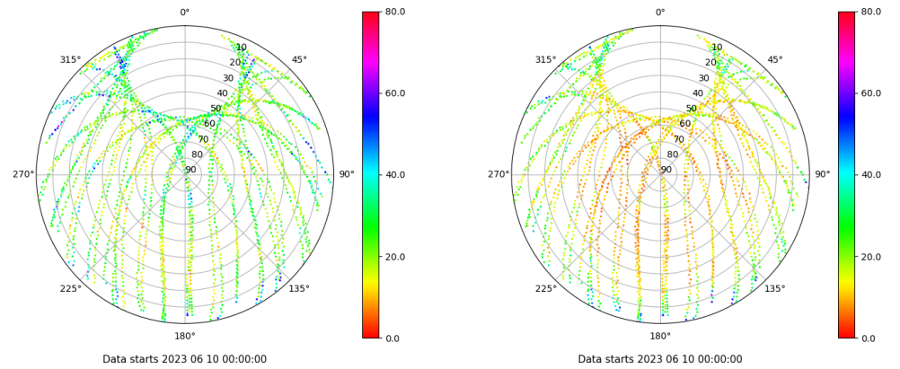
Skyplot for station ALBA. Parameter M1C Data file ALBA00ESP_R_2023161.xtr Skyplot for station ALBA. Parameter M2C Data file ALBA00ESP_R_2023161.xtr
