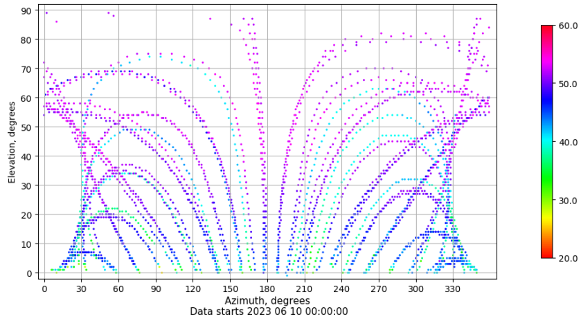
Azimuth-elevation plot for station ALBA. Signal to Noise S1C Data file ALBA00ESP_R_2023161.xtr
