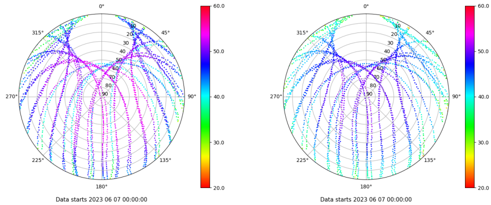
Skyplot for station ALBA. Signal to Noise S1C Data file ALBA00ESP_R_2023158.xtr Skyplot for station ALBA. Signal to Noise S2C Data file ALBA00ESP_R_2023158.xtr
