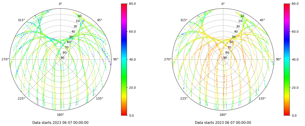
Skyplot for station ALBA. Parameter M1C Data file ALBA00ESP_R_2023158.xtr Skyplot for station ALBA. Parameter M2C Data file ALBA00ESP_R_2023158.xtr
