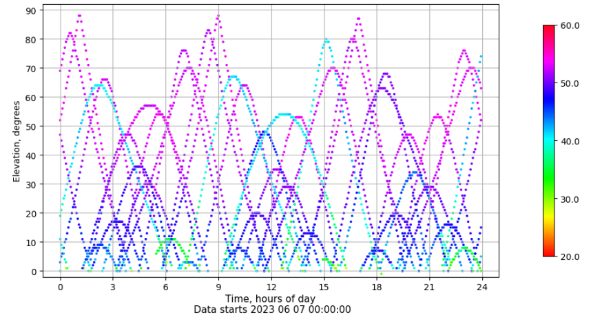
Time-elevation plot for station ALBA. Signal to Noise S1C Data file ALBA00ESP_R_2023158.xtr
