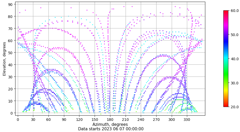
Azimuth-elevation plot for station ALBA. Signal to Noise S1C Data file ALBA00ESP_R_2023158.xtr
