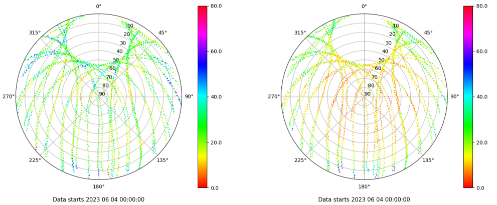
Skyplot for station ALBA. Parameter M1C Data file ALBA00ESP_R_2023155.xtr Skyplot for station ALBA. Parameter M2C Data file ALBA00ESP_R_2023155.xtr
