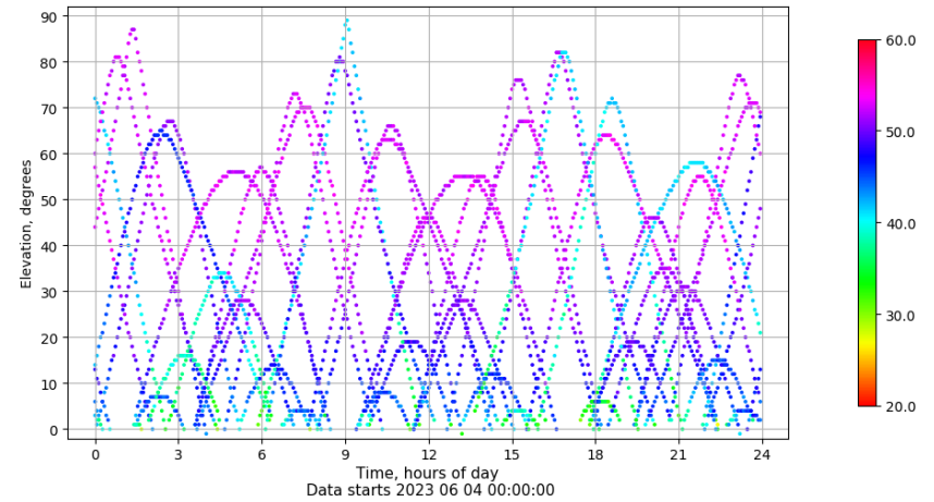
Time-elevation plot for station ALBA. Signal to Noise S1C Data file ALBA00ESP_R_2023155.xtr
