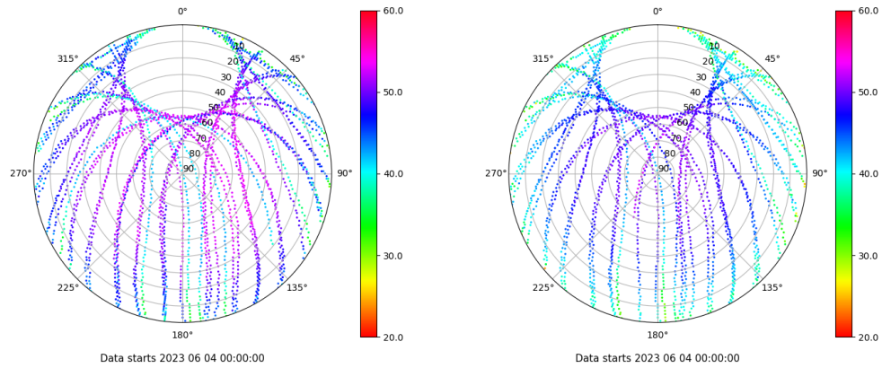
Skyplot for station ALBA. Signal to Noise S1C Data file ALBA00ESP_R_2023155.xtr Skyplot for station ALBA. Signal to Noise S2C Data file ALBA00ESP_R_2023155.xtr
