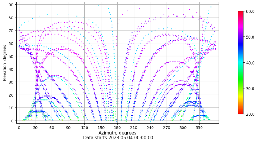
Azimuth-elevation plot for station ALBA. Signal to Noise S1C Data file ALBA00ESP_R_2023155.xtr
