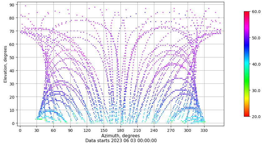
Azimuth-elevation plot for station ALBA. Signal to Noise S1C Data file ALBA00ESP_R_2023154.xtr
