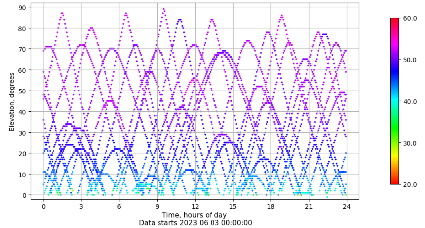
Time-elevation plot for station ALBA. Signal to Noise S1C Data file ALBA00ESP_R_2023154.xtr
