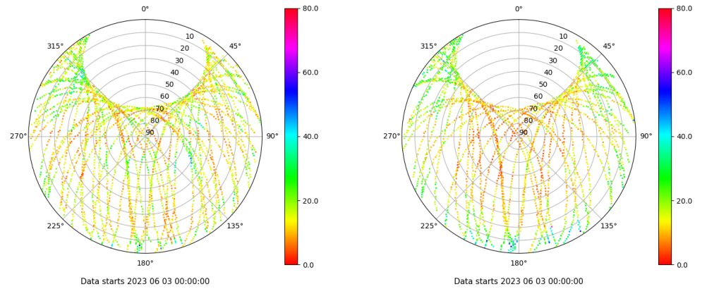
Skyplot for station ALBA. Parameter M1C Data file ALBA00ESP_R_2023154.xtr Skyplot for station ALBA. Parameter M2S Data file ALBA00ESP_R_2023154.xtr
