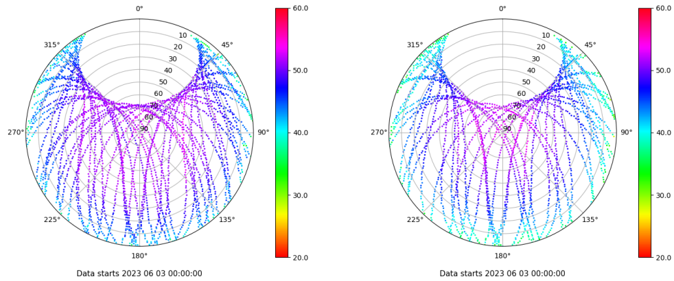
Skyplot for station ALBA. Signal to Noise S1C Data file ALBA00ESP_R_2023154.xtr Skyplot for station ALBA. Signal to Noise S2S Data file ALBA00ESP_R_2023154.xtr
