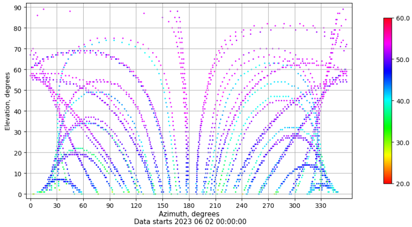
Azimuth-elevation plot for station ALBA. Signal to Noise S1C Data file ALBA00ESP_R_2023153.xtr
