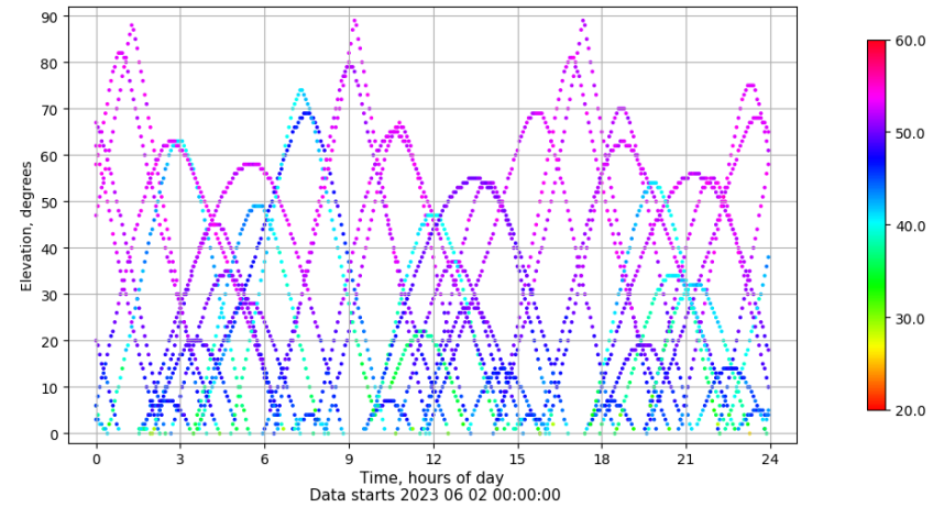
Time-elevation plot for station ALBA. Signal to Noise S1C Data file ALBA00ESP_R_2023153.xtr
