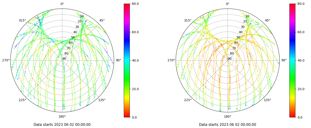
Skyplot for station ALBA. Parameter M1C Data file ALBA00ESP_R_2023153.xtr Skyplot for station ALBA. Parameter M2C Data file ALBA00ESP_R_2023153.xtr
