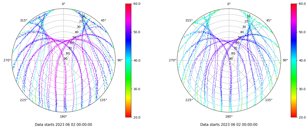
Skyplot for station ALBA. Signal to Noise S1C Data file ALBA00ESP_R_2023153.xtr Skyplot for station ALBA. Signal to Noise S2C Data file ALBA00ESP_R_2023153.xtr
