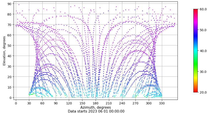
Azimuth-elevation plot for station ALBA. Signal to Noise S1C Data file ALBA00ESP_R_2023152.xtr
