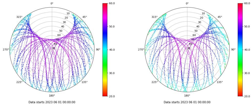
Skyplot for station ALBA. Signal to Noise S1C Data file ALBA00ESP_R_2023152.xtr Skyplot for station ALBA. Signal to Noise S2S Data file ALBA00ESP_R_2023152.xtr
