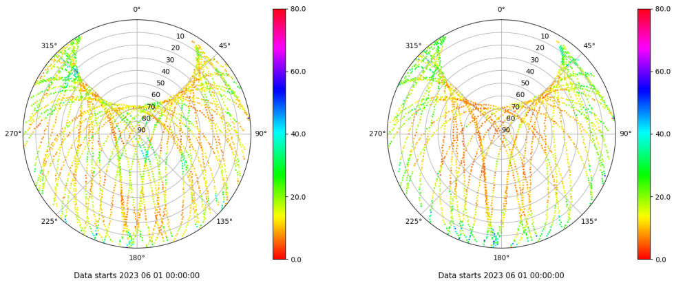
Skyplot for station ALBA. Parameter M1C Data file ALBA00ESP_R_2023152.xtr Skyplot for station ALBA. Parameter M2S Data file ALBA00ESP_R_2023152.xtr
