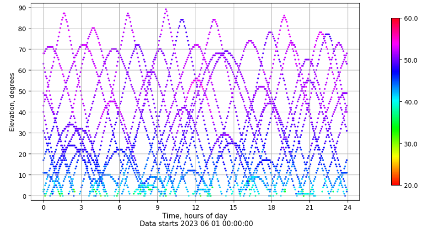
Time-elevation plot for station ALBA. Signal to Noise S1C Data file ALBA00ESP_R_2023152.xtr
