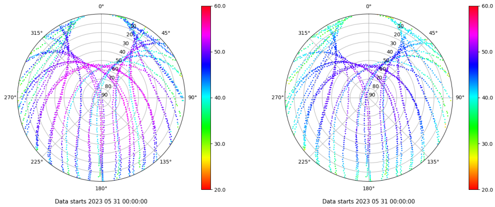
Skyplot for station ALBA. Signal to Noise S1C Data file ALBA00ESP_R_2023151.xtr Skyplot for station ALBA. Signal to Noise S2C Data file ALBA00ESP_R_2023151.xtr
