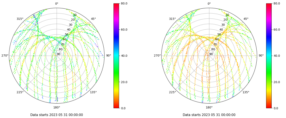
Skyplot for station ALBA. Parameter M1C Data file ALBA00ESP_R_2023151.xtr Skyplot for station ALBA. Parameter M2C Data file ALBA00ESP_R_2023151.xtr
