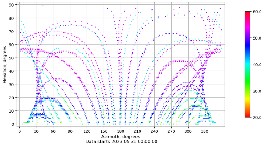
Azimuth-elevation plot for station ALBA. Signal to Noise S1C Data file ALBA00ESP_R_2023151.xtr
