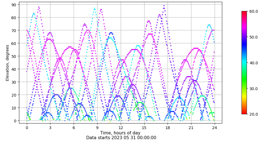
Time-elevation plot for station ALBA. Signal to Noise S1C Data file ALBA00ESP_R_2023151.xtr
