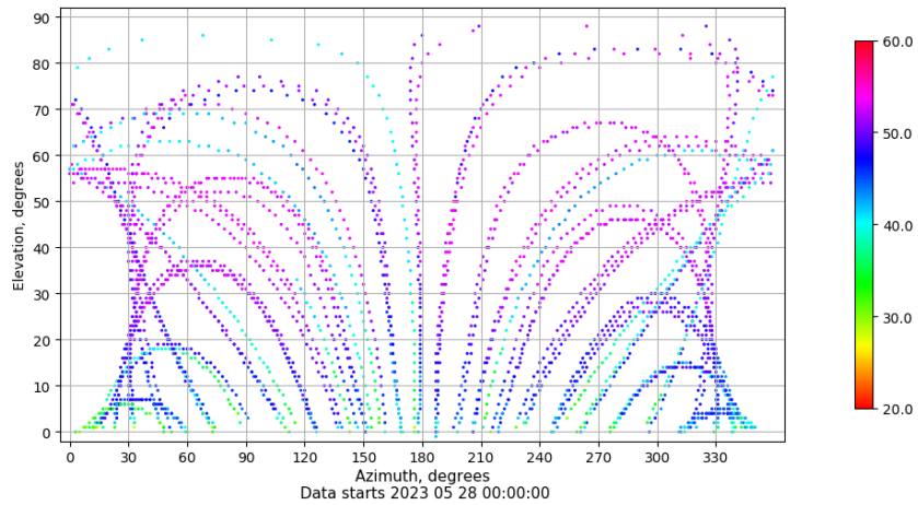
Azimuth-elevation plot for station ALBA. Signal to Noise S1C Data file ALBA00ESP_R_2023148.xtr
