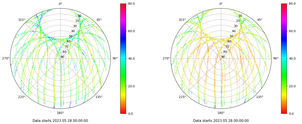
Skyplot for station ALBA. Parameter M1C Data file ALBA00ESP_R_2023148.xtr Skyplot for station ALBA. Parameter M2C Data file ALBA00ESP_R_2023148.xtr
