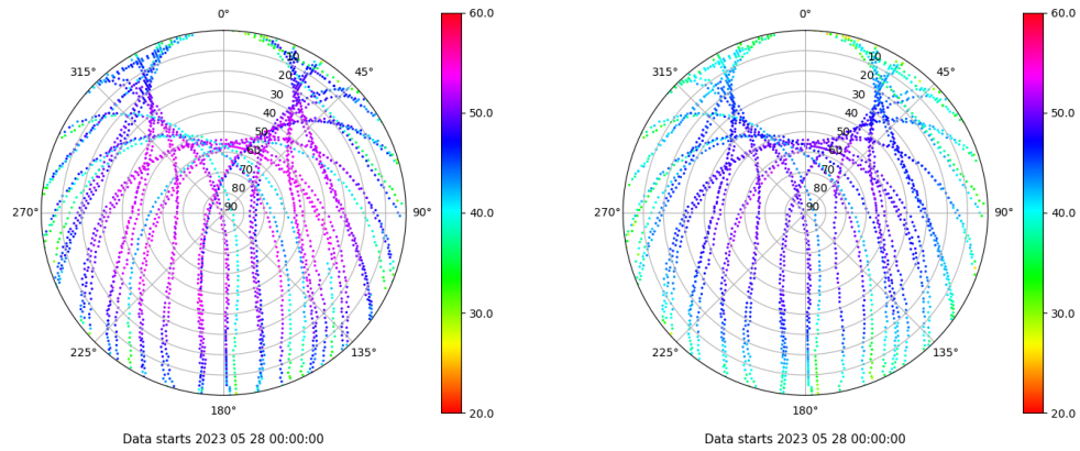
Skyplot for station ALBA. Signal to Noise S1C Data file ALBA00ESP_R_2023148.xtr Skyplot for station ALBA. Signal to Noise S2C Data file ALBA00ESP_R_2023148.xtr
