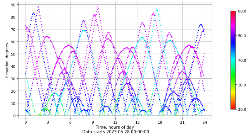
Time-elevation plot for station ALBA. Signal to Noise S1C Data file ALBA00ESP_R_2023148.xtr
