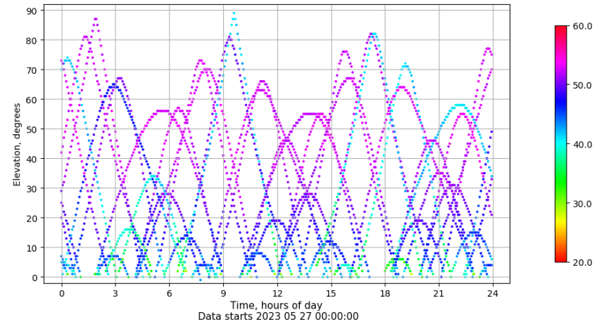
Time-elevation plot for station ALBA. Signal to Noise S1C Data file ALBA00ESP_R_2023147.xtr
