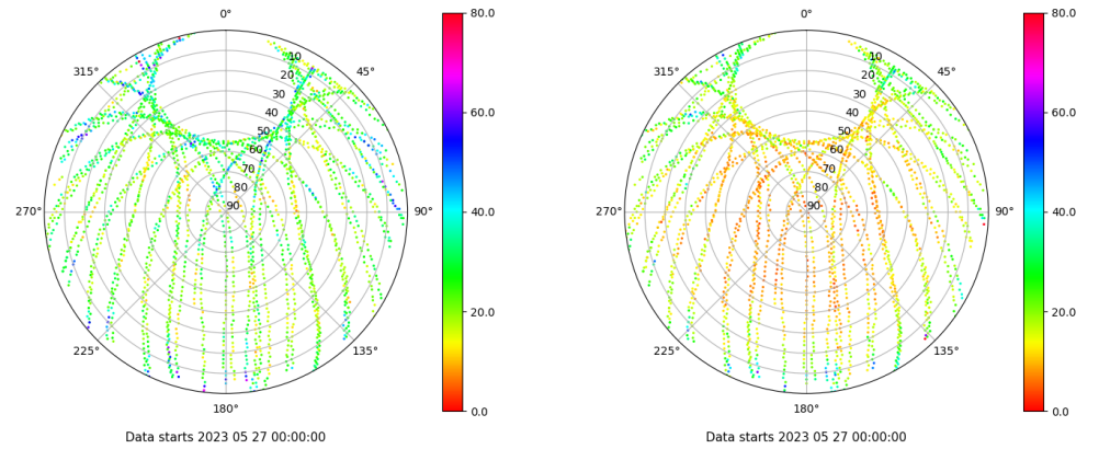
Skyplot for station ALBA. Parameter M1C Data file ALBA00ESP_R_2023147.xtr Skyplot for station ALBA. Parameter M2C Data file ALBA00ESP_R_2023147.xtr
