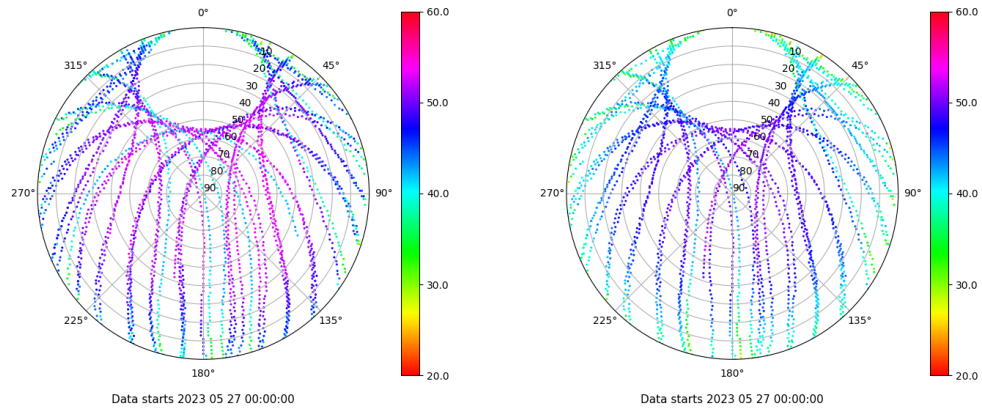
Skyplot for station ALBA. Signal to Noise S1C Data file ALBA00ESP_R_2023147.xtr Skyplot for station ALBA. Signal to Noise S2C Data file ALBA00ESP_R_2023147.xtr
