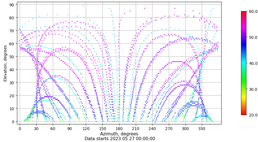
Azimuth-elevation plot for station ALBA. Signal to Noise S1C Data file ALBA00ESP_R_2023147.xtr
