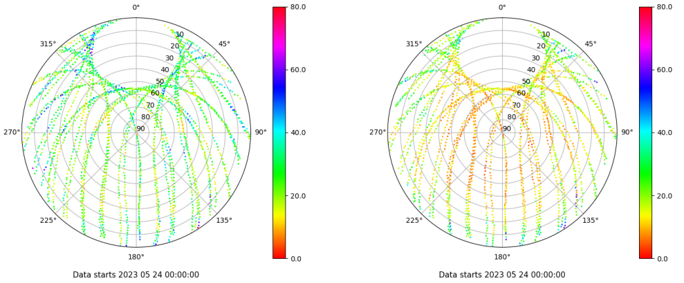
Skyplot for station ALBA. Parameter M1C Data file ALBA00ESP_R_2023144.xtr Skyplot for station ALBA. Parameter M2C Data file ALBA00ESP_R_2023144.xtr
