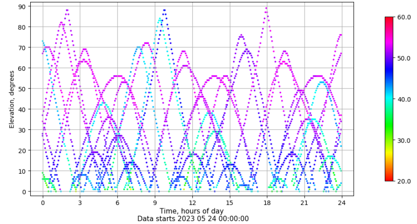
Time-elevation plot for station ALBA. Signal to Noise S1C Data file ALBA00ESP_R_2023144.xtr
