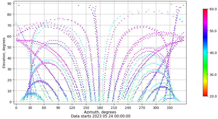
Azimuth-elevation plot for station ALBA. Signal to Noise S1C Data file ALBA00ESP_R_2023144.xtr
