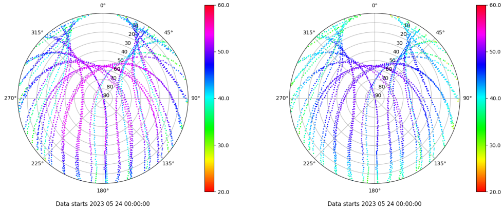
Skyplot for station ALBA. Signal to Noise S1C Data file ALBA00ESP_R_2023144.xtr Skyplot for station ALBA. Signal to Noise S2C Data file ALBA00ESP_R_2023144.xtr
