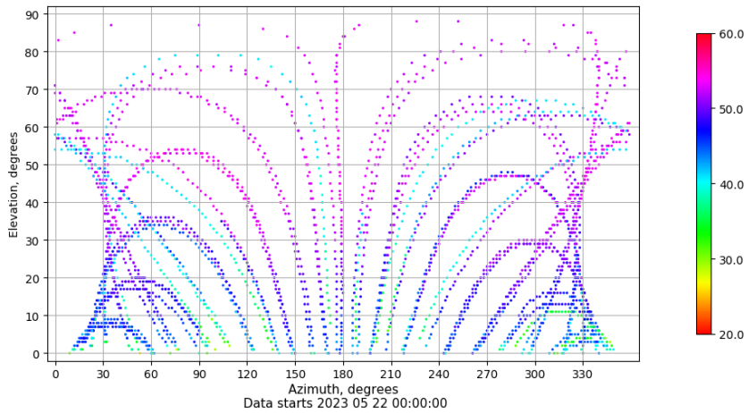
Azimuth-elevation plot for station ALBA. Signal to Noise S1C Data file ALBA00ESP_R_2023142.xtr
