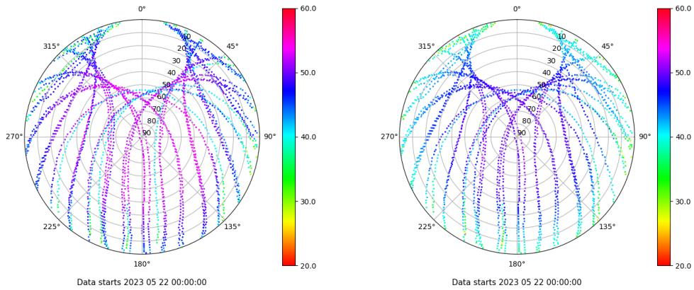
Skyplot for station ALBA. Signal to Noise S1C Data file ALBA00ESP_R_2023142.xtr Skyplot for station ALBA. Signal to Noise S2C Data file ALBA00ESP_R_2023142.xtr
