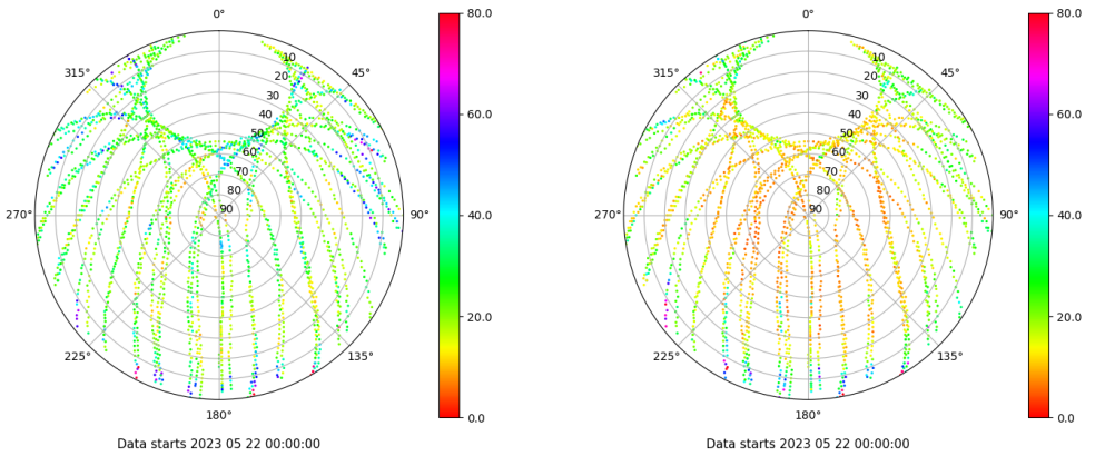
Skyplot for station ALBA. Parameter M1C Data file ALBA00ESP_R_2023142.xtr Skyplot for station ALBA. Parameter M2C Data file ALBA00ESP_R_2023142.xtr
