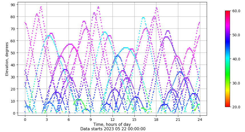
Time-elevation plot for station ALBA. Signal to Noise S1C Data file ALBA00ESP_R_2023142.xtr
