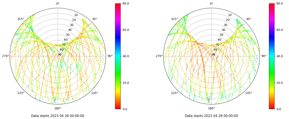
Skyplot for station ALBA. Parameter M1C Data file ALBA00ESP_R_2023118.xtr Skyplot for station ALBA. Parameter M2S Data file ALBA00ESP_R_2023118.xtr
