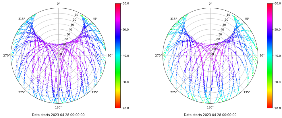
Skyplot for station ALBA. Signal to Noise S1C Data file ALBA00ESP_R_2023118.xtr Skyplot for station ALBA. Signal to Noise S2S Data file ALBA00ESP_R_2023118.xtr
