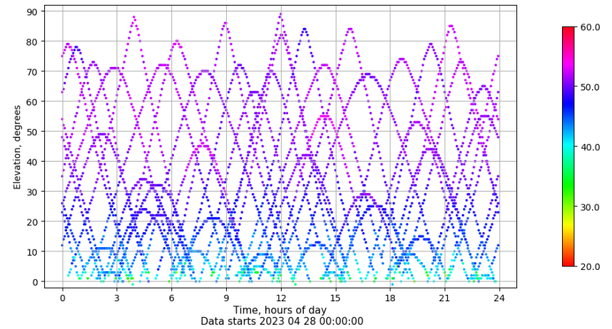
Time-elevation plot for station ALBA. Signal to Noise S1C Data file ALBA00ESP_R_2023118.xtr
