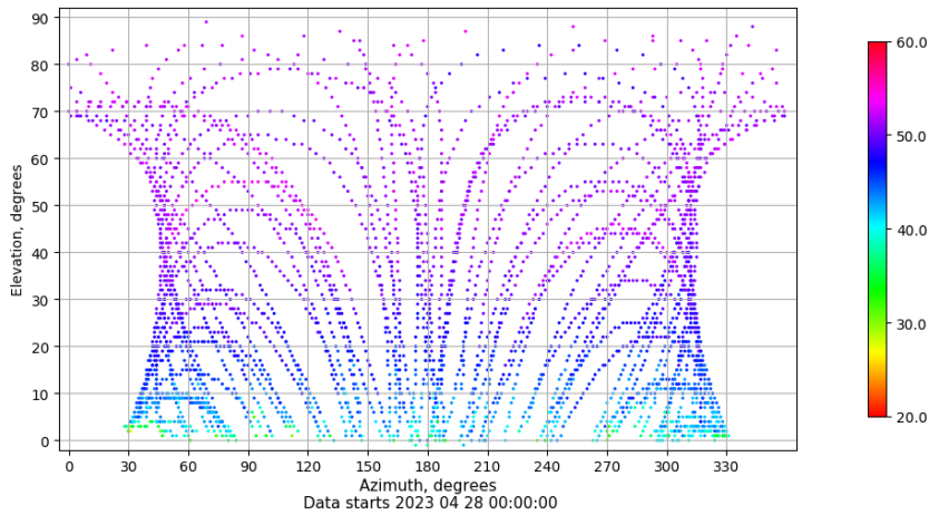
Azimuth-elevation plot for station ALBA. Signal to Noise S1C Data file ALBA00ESP_R_2023118.xtr
