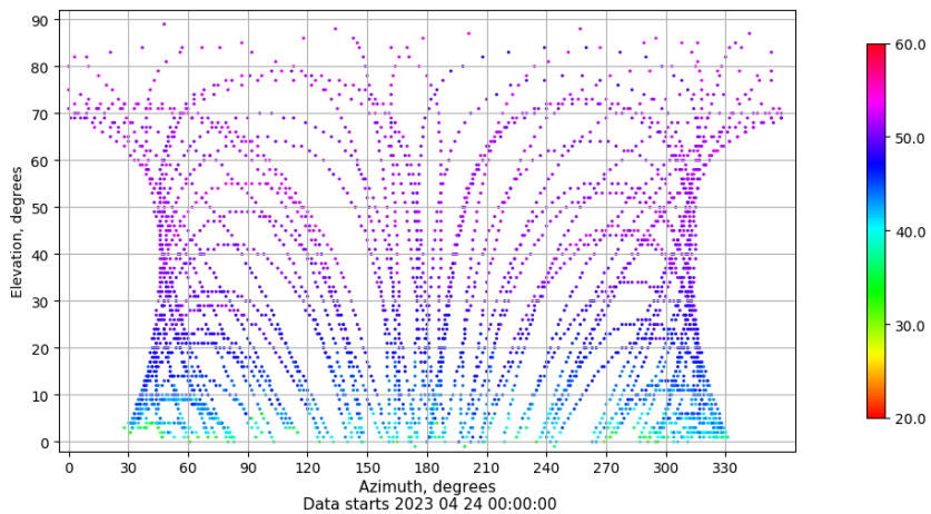
Azimuth-elevation plot for station ALBA. Signal to Noise S1C Data file ALBA00ESP_R_2023114.xtr
