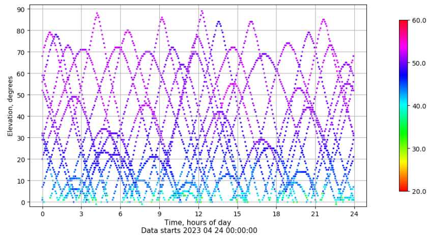
Time-elevation plot for station ALBA. Signal to Noise S1C Data file ALBA00ESP_R_2023114.xtr
