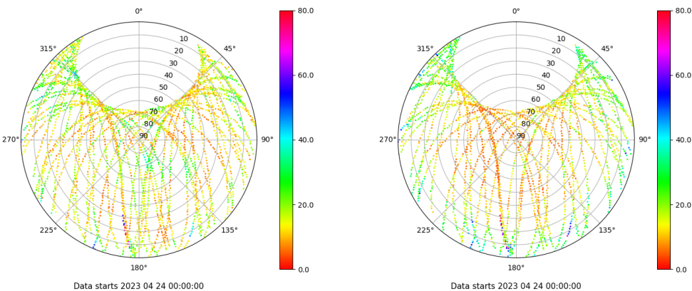
Skyplot for station ALBA. Parameter M1C Data file ALBA00ESP_R_2023114.xtr Skyplot for station ALBA. Parameter M2S Data file ALBA00ESP_R_2023114.xtr
