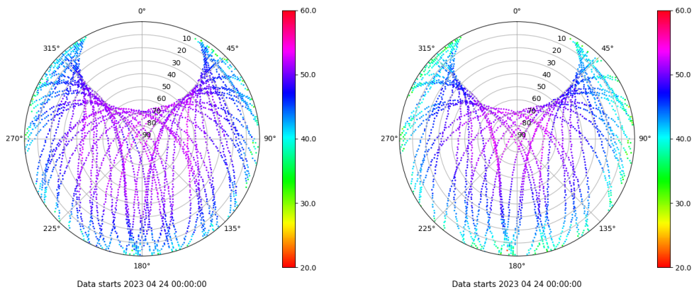
Skyplot for station ALBA. Signal to Noise S1C Data file ALBA00ESP_R_2023114.xtr Skyplot for station ALBA. Signal to Noise S2S Data file ALBA00ESP_R_2023114.xtr
