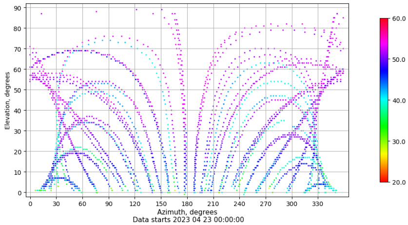
Azimuth-elevation plot for station ALBA. Signal to Noise S1C Data file ALBA00ESP_R_2023113.xtr
