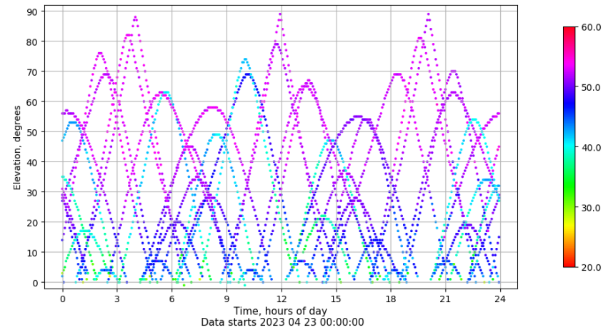
Time-elevation plot for station ALBA. Signal to Noise S1C Data file ALBA00ESP_R_2023113.xtr
