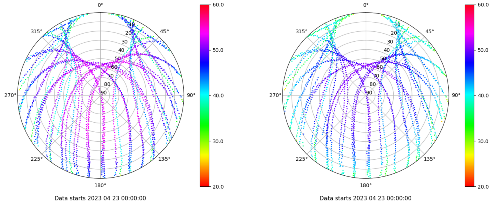
Skyplot for station ALBA. Signal to Noise S1C Data file ALBA00ESP_R_2023113.xtr Skyplot for station ALBA. Signal to Noise S2C Data file ALBA00ESP_R_2023113.xtr
