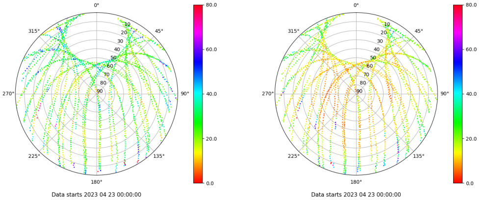
Skyplot for station ALBA. Parameter M1C Data file ALBA00ESP_R_2023113.xtr Skyplot for station ALBA. Parameter M2C Data file ALBA00ESP_R_2023113.xtr
