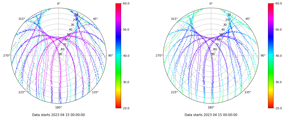
Skyplot for station ALBA. Signal to Noise S1C Data file ALBA00ESP_R_2023105.xtr Skyplot for station ALBA. Signal to Noise S2C Data file ALBA00ESP_R_2023105.xtr
