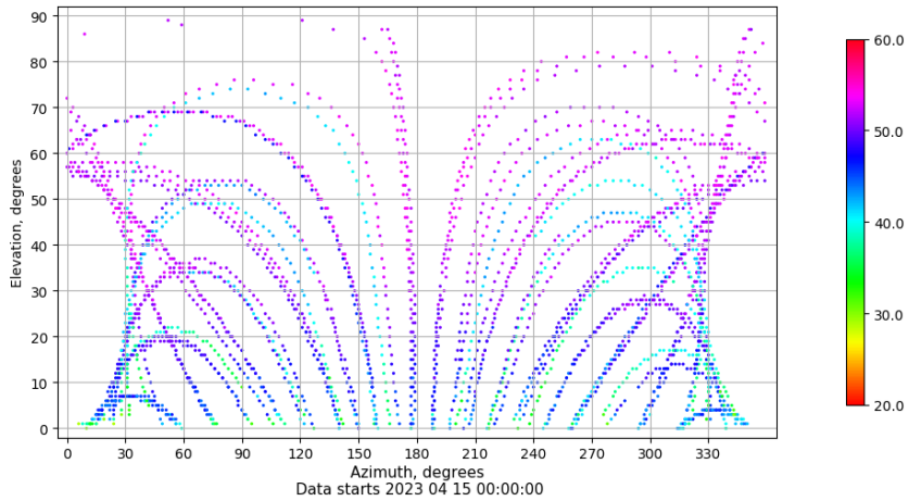
Azimuth-elevation plot for station ALBA. Signal to Noise S1C Data file ALBA00ESP_R_2023105.xtr
