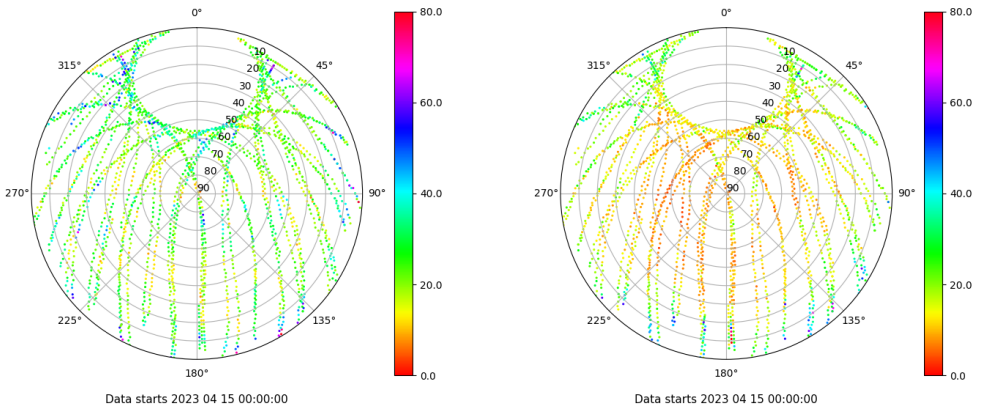
Skyplot for station ALBA. Parameter M1C Data file ALBA00ESP_R_2023105.xtr Skyplot for station ALBA. Parameter M2C Data file ALBA00ESP_R_2023105.xtr
