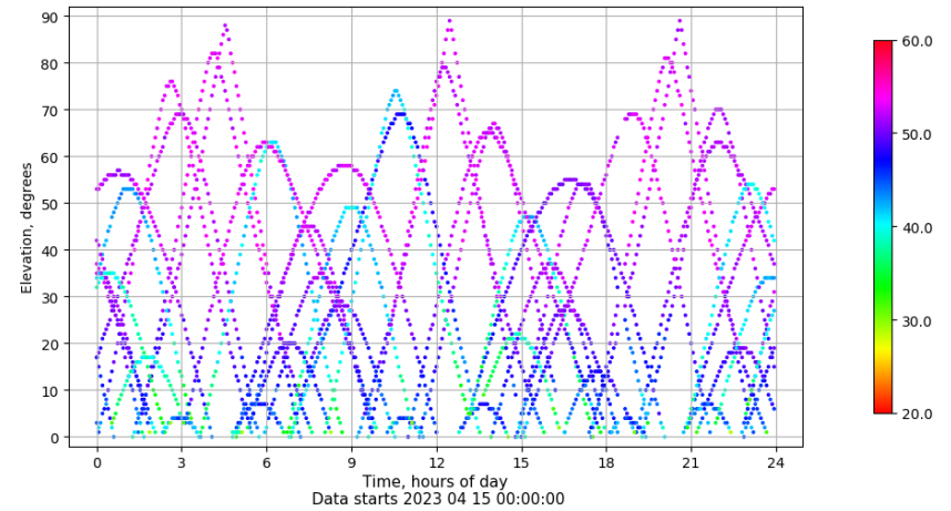
Time-elevation plot for station ALBA. Signal to Noise S1C Data file ALBA00ESP_R_2023105.xtr
