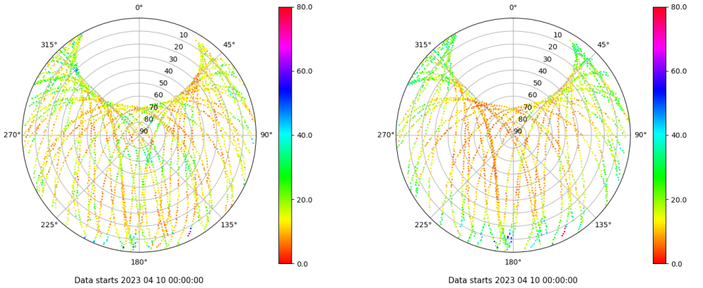
Skyplot for station ALBA. Parameter M1C Data file ALBA00ESP_R_2023100.xtr Skyplot for station ALBA. Parameter M2S Data file ALBA00ESP_R_2023100.xtr
