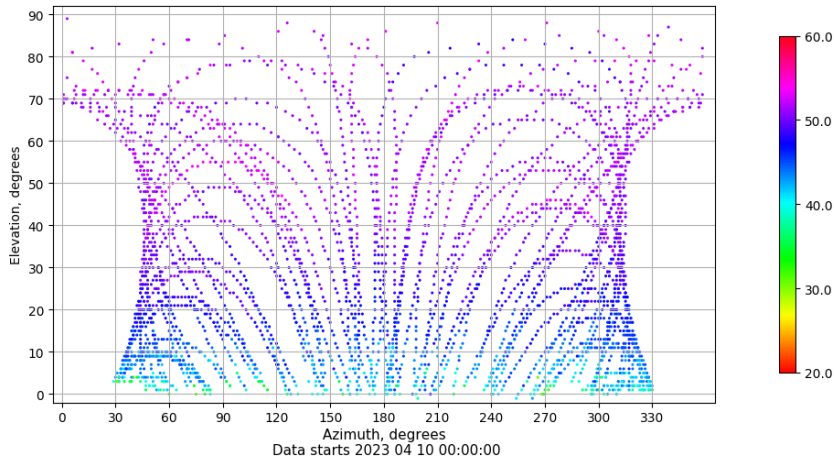
Azimuth-elevation plot for station ALBA. Signal to Noise S1C Data file ALBA00ESP_R_2023100.xtr
