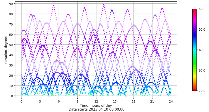
Time-elevation plot for station ALBA. Signal to Noise S1C Data file ALBA00ESP_R_2023100.xtr
