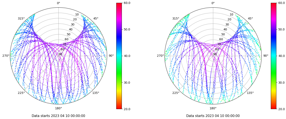
Skyplot for station ALBA. Signal to Noise S1C Data file ALBA00ESP_R_2023100.xtr Skyplot for station ALBA. Signal to Noise S2S Data file ALBA00ESP_R_2023100.xtr
