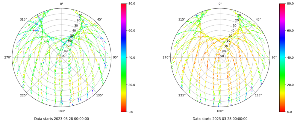
Skyplot for station ALBA. Parameter M1C Data file ALBA00ESP_R_2023087.xtr Skyplot for station ALBA. Parameter M2C Data file ALBA00ESP_R_2023087.xtr
