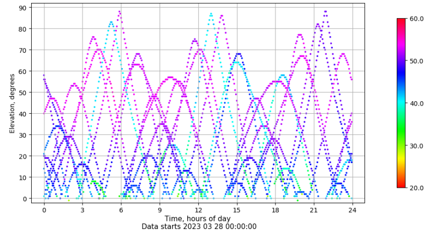
Time-elevation plot for station ALBA. Signal to Noise S1C Data file ALBA00ESP_R_2023087.xtr
