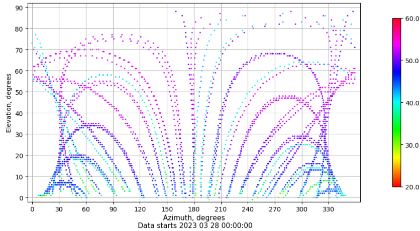
Azimuth-elevation plot for station ALBA. Signal to Noise S1C Data file ALBA00ESP_R_2023087.xtr
