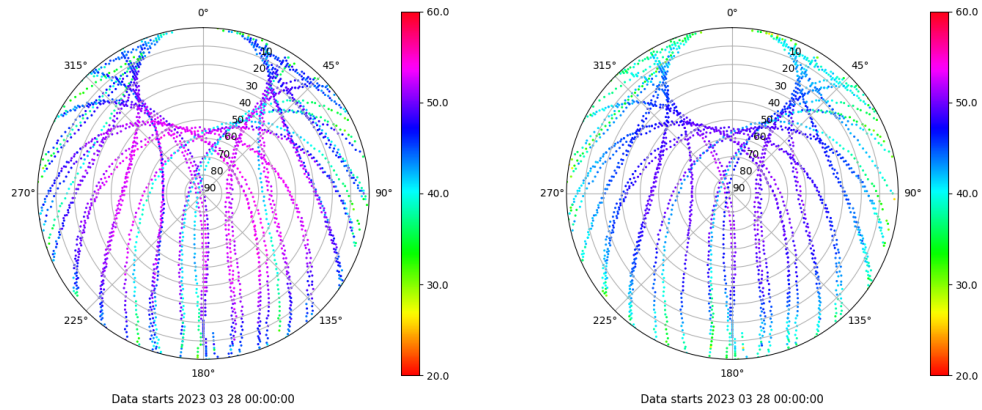
Skyplot for station ALBA. Signal to Noise S1C Data file ALBA00ESP_R_2023087.xtr Skyplot for station ALBA. Signal to Noise S2C Data file ALBA00ESP_R_2023087.xtr
