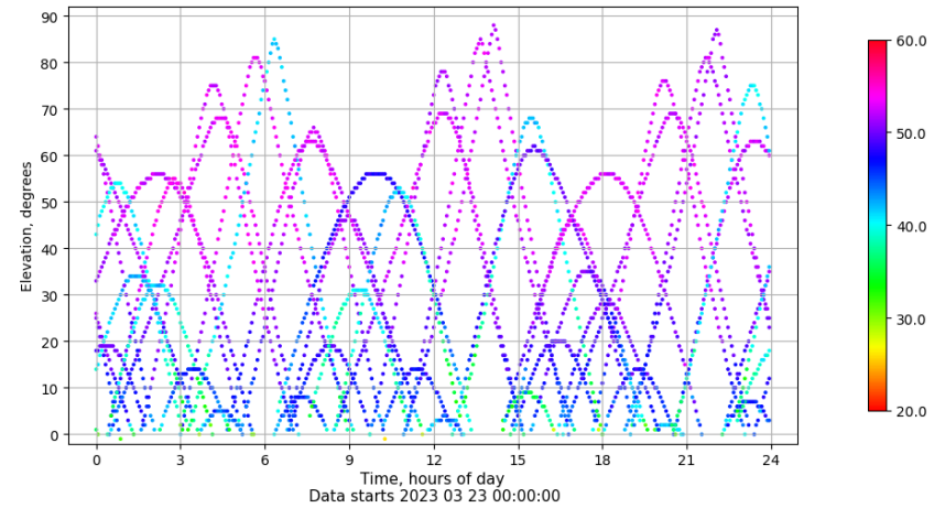
Time-elevation plot for station ALBA. Signal to Noise S1C Data file ALBA00ESP_R_2023082.xtr
