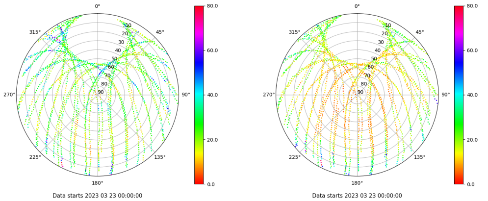
Skyplot for station ALBA. Parameter M1C Data file ALBA00ESP_R_2023082.xtr Skyplot for station ALBA. Parameter M2C Data file ALBA00ESP_R_2023082.xtr
