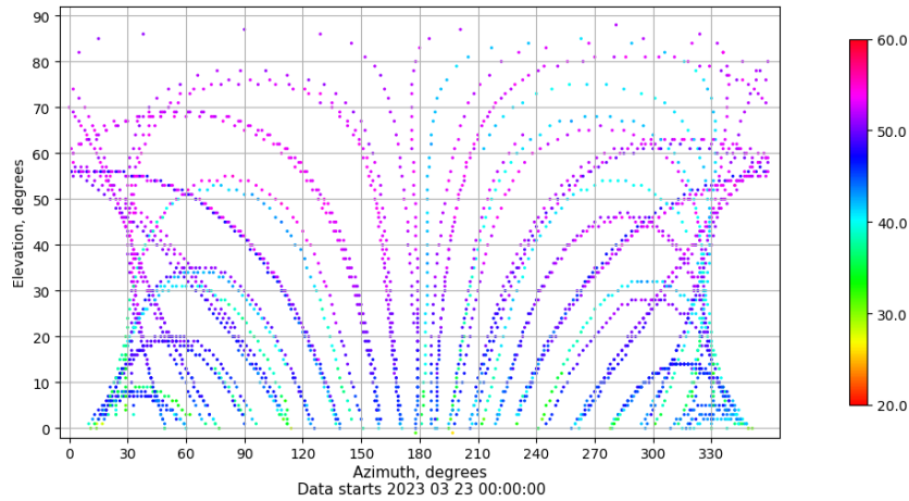
Azimuth-elevation plot for station ALBA. Signal to Noise S1C Data file ALBA00ESP_R_2023082.xtr
