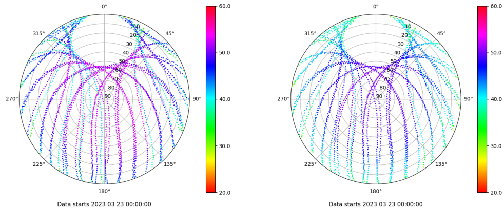
Skyplot for station ALBA. Signal to Noise S1C Data file ALBA00ESP_R_2023082.xtr Skyplot for station ALBA. Signal to Noise S2C Data file ALBA00ESP_R_2023082.xtr
