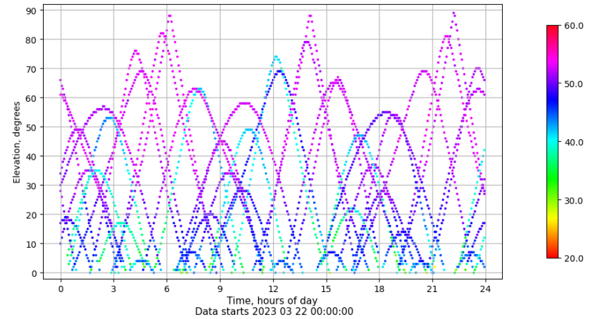
Time-elevation plot for station ALBA. Signal to Noise S1C Data file ALBA00ESP_R_2023081.xtr
