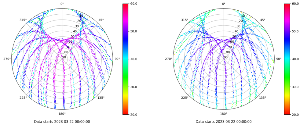
Skyplot for station ALBA. Signal to Noise S1C Data file ALBA00ESP_R_2023081.xtr Skyplot for station ALBA. Signal to Noise S2C Data file ALBA00ESP_R_2023081.xtr
