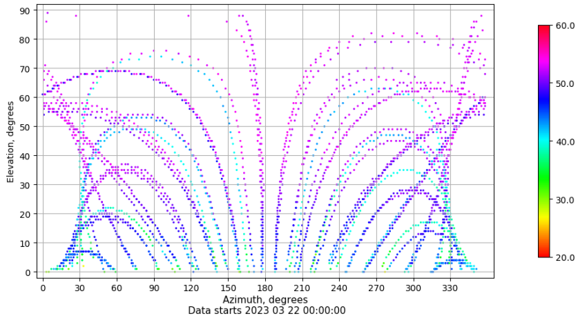
Azimuth-elevation plot for station ALBA. Signal to Noise S1C Data file ALBA00ESP_R_2023081.xtr
