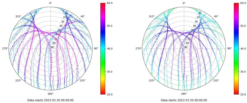
Skyplot for station ALBA. Signal to Noise S1C Data file ALBA00ESP_R_2023079.xtr Skyplot for station ALBA. Signal to Noise S2C Data file ALBA00ESP_R_2023079.xtr
