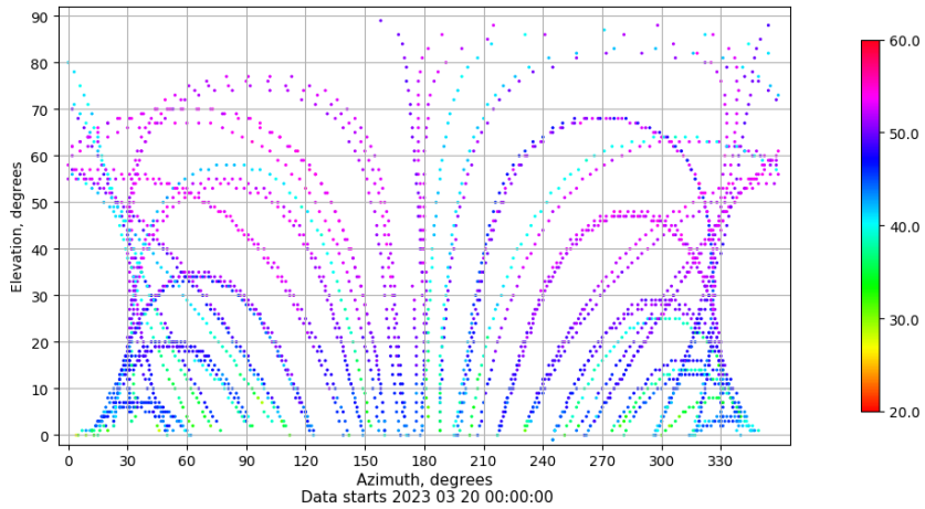
Azimuth-elevation plot for station ALBA. Signal to Noise S1C Data file ALBA00ESP_R_2023079.xtr
