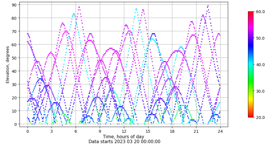
Time-elevation plot for station ALBA. Signal to Noise S1C Data file ALBA00ESP_R_2023079.xtr
