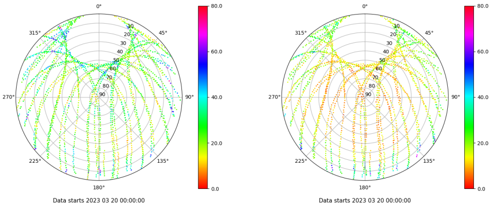
Skyplot for station ALBA. Parameter M1C Data file ALBA00ESP_R_2023079.xtr Skyplot for station ALBA. Parameter M2C Data file ALBA00ESP_R_2023079.xtr
