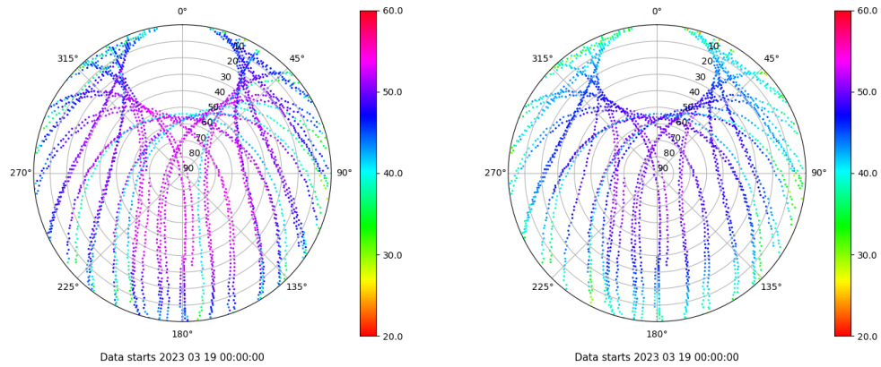
Skyplot for station ALBA. Signal to Noise S1C Data file ALBA00ESP_R_2023078.xtr Skyplot for station ALBA. Signal to Noise S2C Data file ALBA00ESP_R_2023078.xtr
