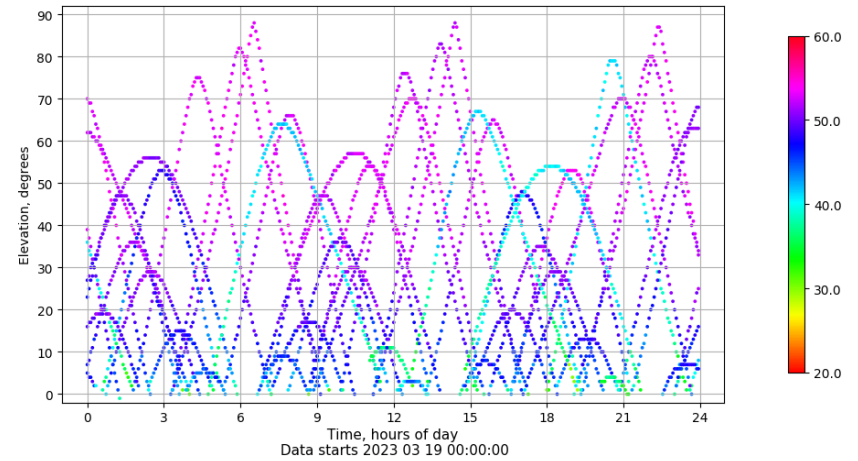
Time-elevation plot for station ALBA. Signal to Noise S1C Data file ALBA00ESP_R_2023078.xtr
