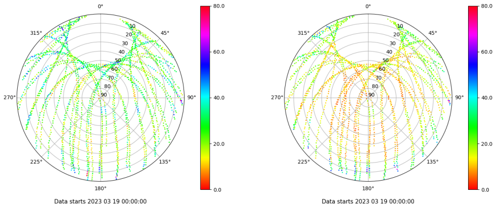
Skyplot for station ALBA. Parameter M1C Data file ALBA00ESP_R_2023078.xtr Skyplot for station ALBA. Parameter M2C Data file ALBA00ESP_R_2023078.xtr
