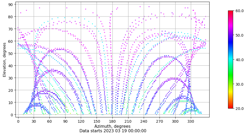
Azimuth-elevation plot for station ALBA. Signal to Noise S1C Data file ALBA00ESP_R_2023078.xtr
