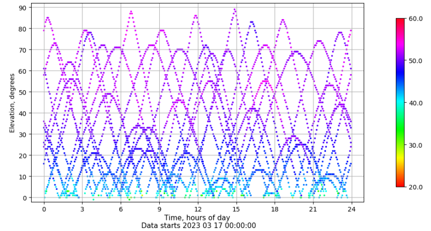
Time-elevation plot for station ALBA. Signal to Noise S1C Data file ALBA00ESP_R_2023076.xtr
