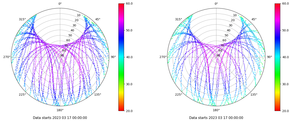
Skyplot for station ALBA. Signal to Noise S1C Data file ALBA00ESP_R_2023076.xtr Skyplot for station ALBA. Signal to Noise S2S Data file ALBA00ESP_R_2023076.xtr
