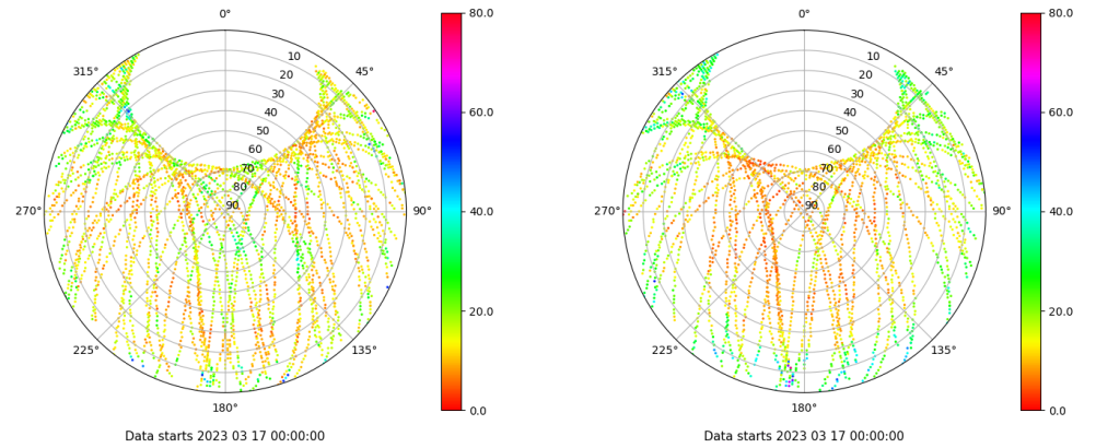
Skyplot for station ALBA. Parameter M1C Data file ALBA00ESP_R_2023076.xtr Skyplot for station ALBA. Parameter M2S Data file ALBA00ESP_R_2023076.xtr
