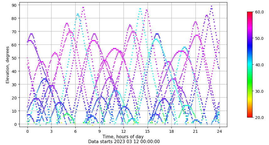
Time-elevation plot for station ALBA. Signal to Noise S1C Data file ALBA00ESP_R_2023071.xtr
