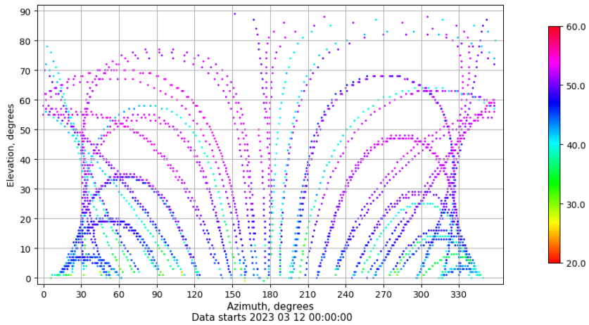
Azimuth-elevation plot for station ALBA. Signal to Noise S1C Data file ALBA00ESP_R_2023071.xtr
