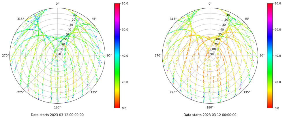
Skyplot for station ALBA. Parameter M1C Data file ALBA00ESP_R_2023071.xtr Skyplot for station ALBA. Parameter M2C Data file ALBA00ESP_R_2023071.xtr
