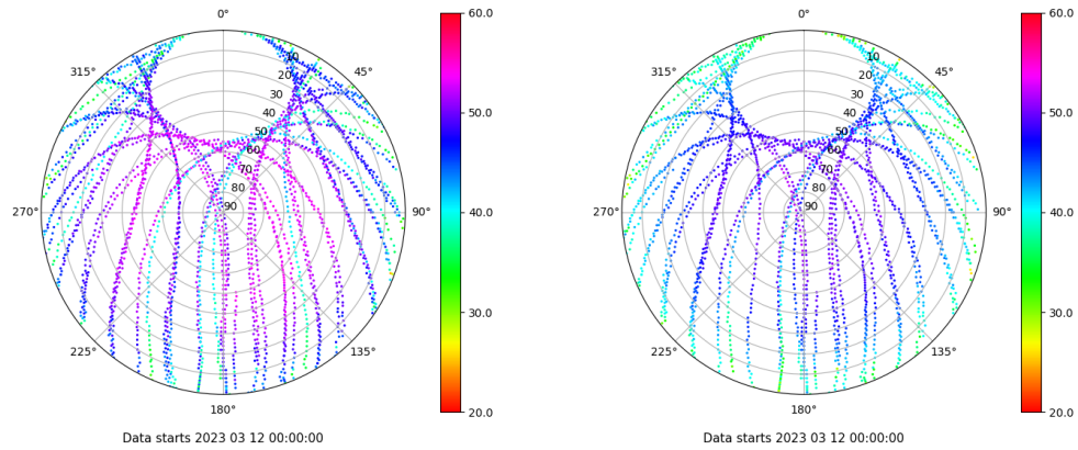
Skyplot for station ALBA. Signal to Noise S1C Data file ALBA00ESP_R_2023071.xtr Skyplot for station ALBA. Signal to Noise S2C Data file ALBA00ESP_R_2023071.xtr
