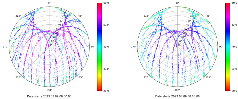
Skyplot for station ALBA. Signal to Noise S1C Data file ALBA00ESP_R_2023068.xtr Skyplot for station ALBA. Signal to Noise S2C Data file ALBA00ESP_R_2023068.xtr
