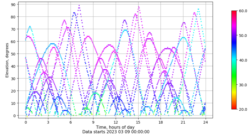
Time-elevation plot for station ALBA. Signal to Noise S1C Data file ALBA00ESP_R_2023068.xtr
