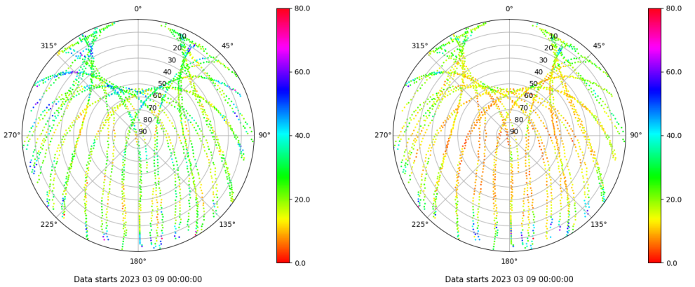
Skyplot for station ALBA. Parameter M1C Data file ALBA00ESP_R_2023068.xtr Skyplot for station ALBA. Parameter M2C Data file ALBA00ESP_R_2023068.xtr
