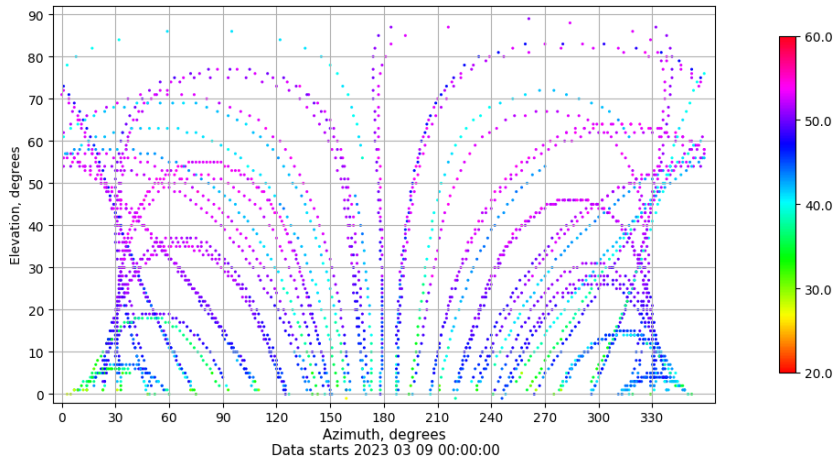
Azimuth-elevation plot for station ALBA. Signal to Noise S1C Data file ALBA00ESP_R_2023068.xtr
